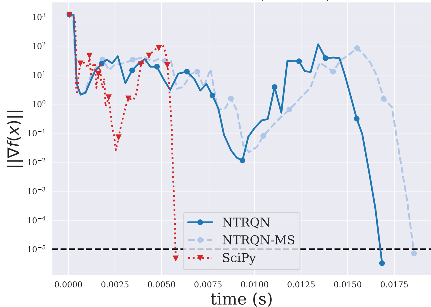
LSC1LS ( n = 3 )
