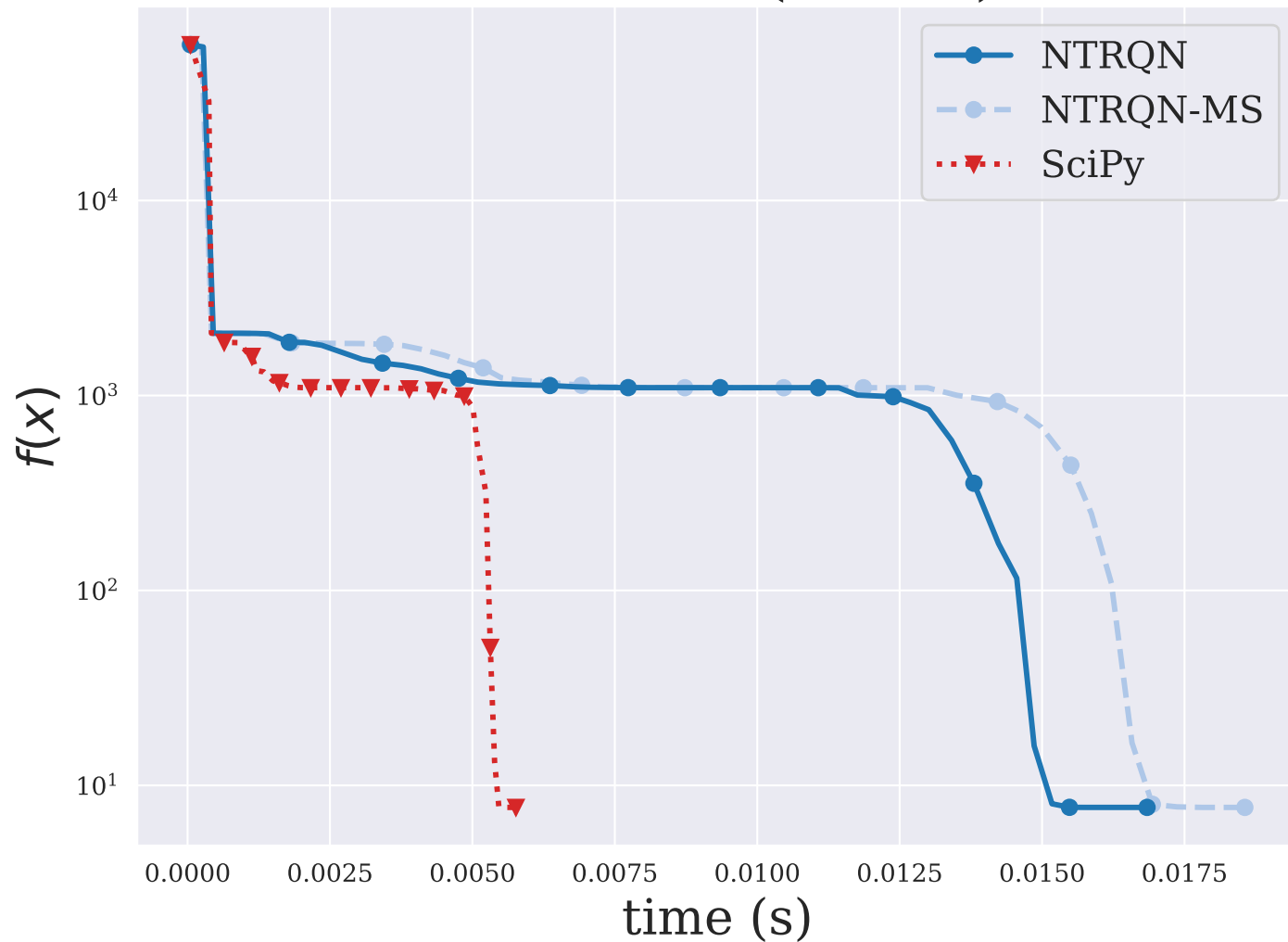
LSC1LS ( n = 3 )
