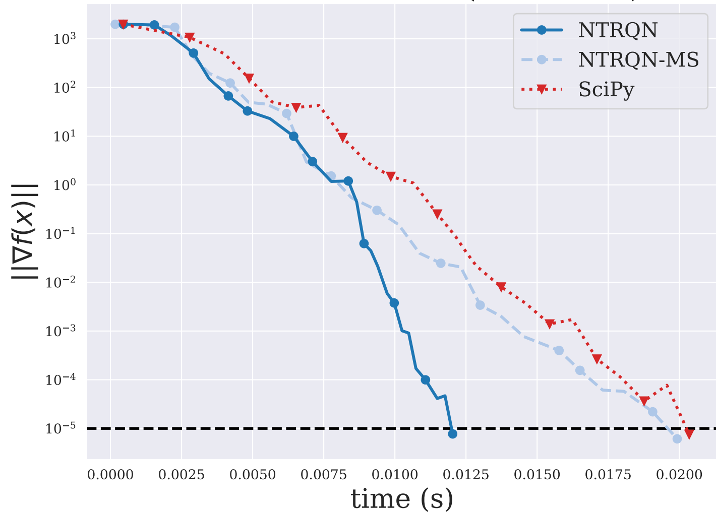
LUKSAN15LS ( n = 100 )
