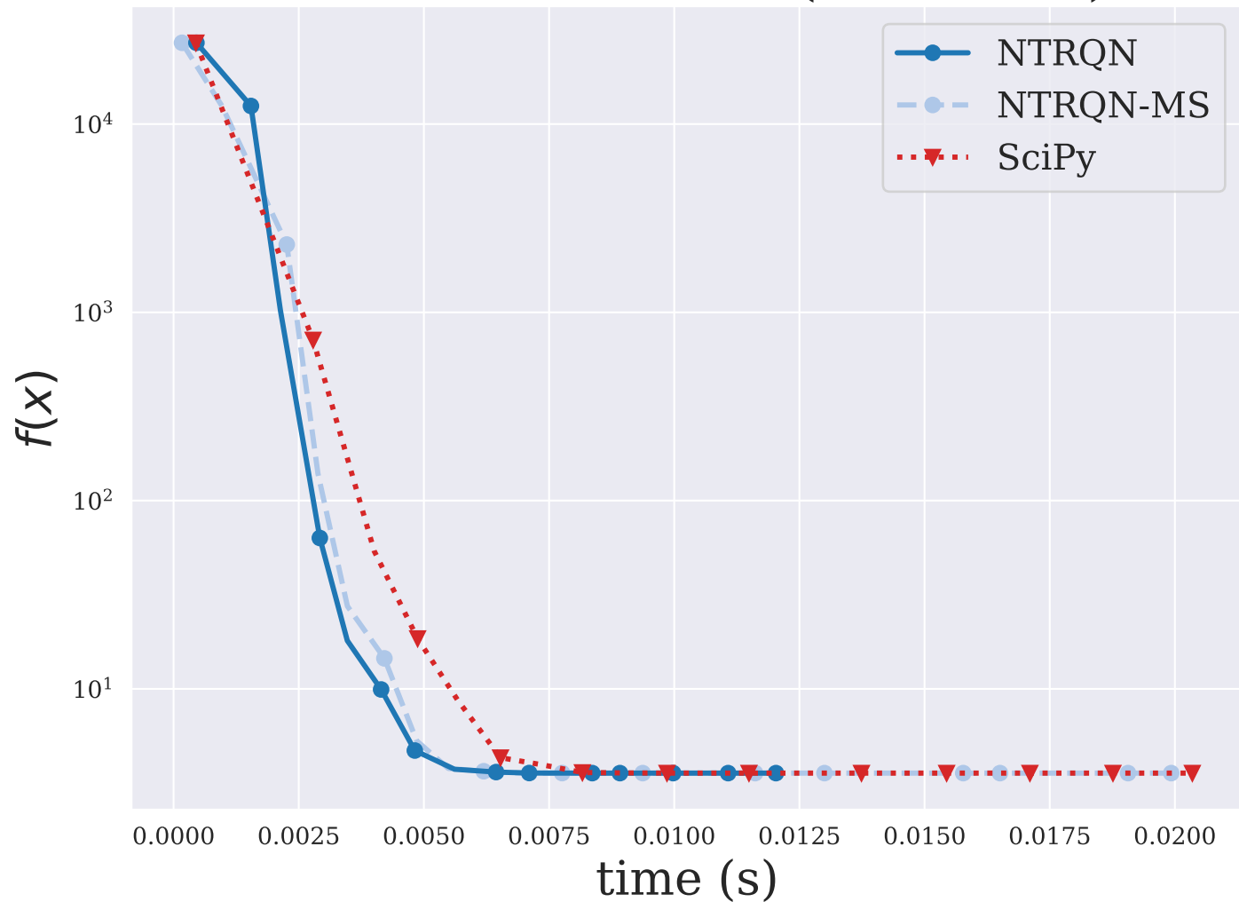
LUKSAN15LS ( n = 100 )
