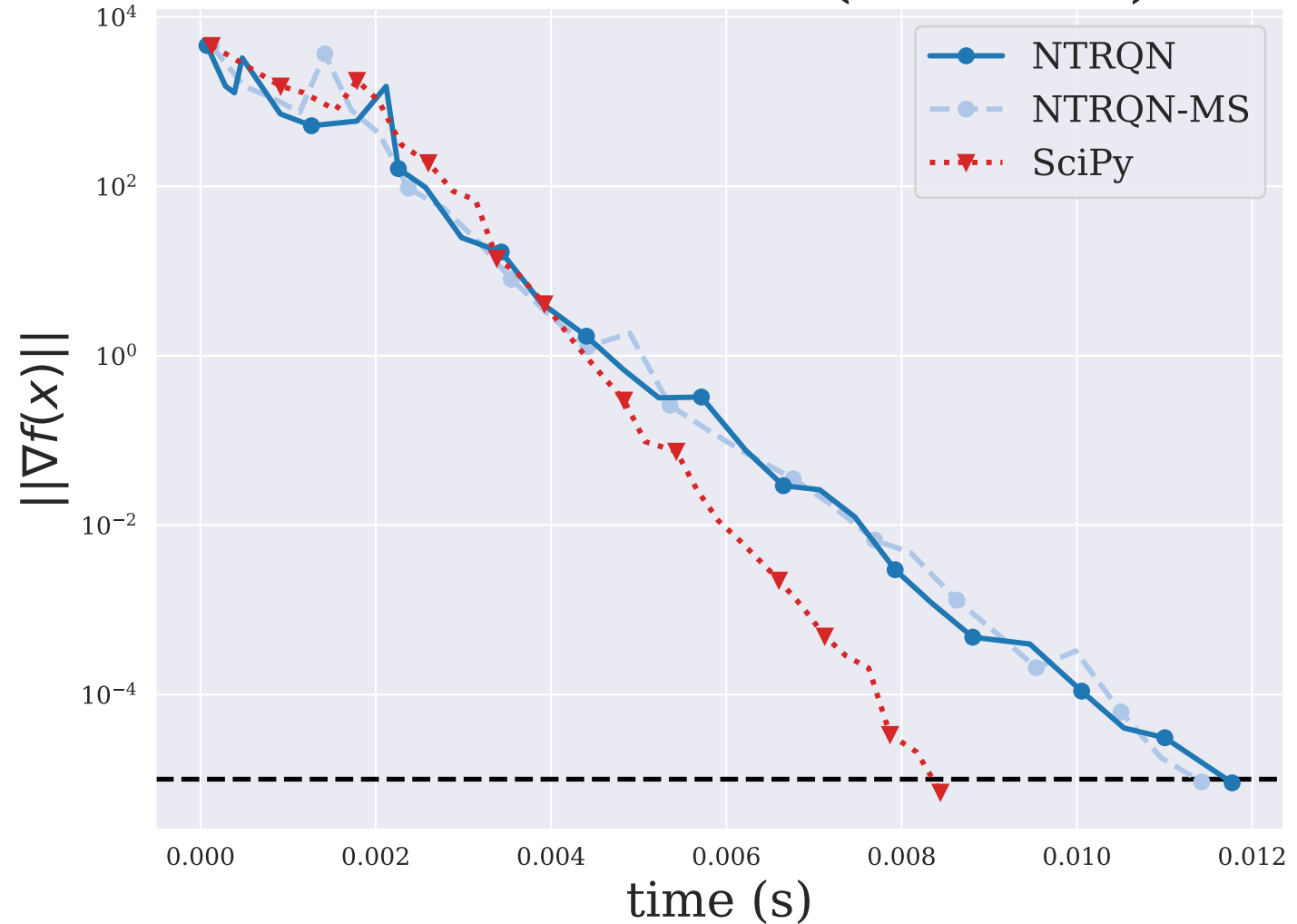
LUKSAN16LS ( n = 100 )
