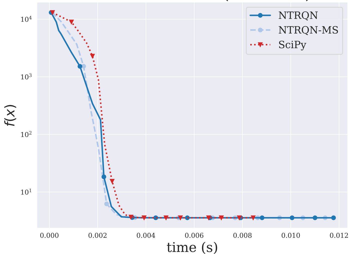
LUKSAN16LS ( n = 100 )
