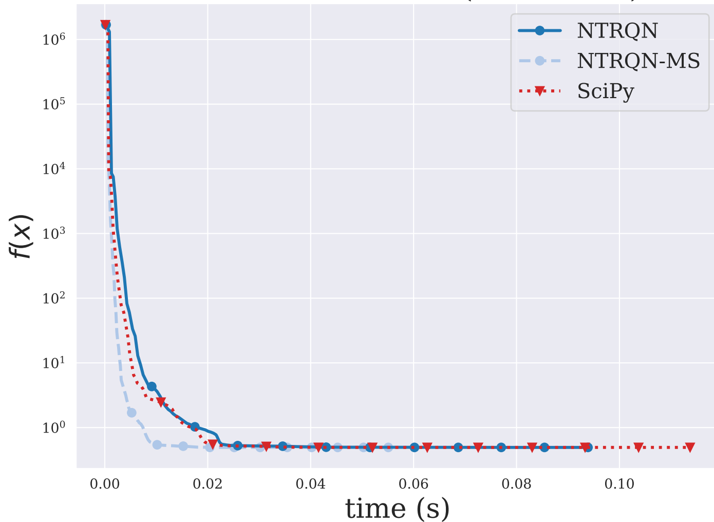
LUKSAN17LS ( n = 100 )
