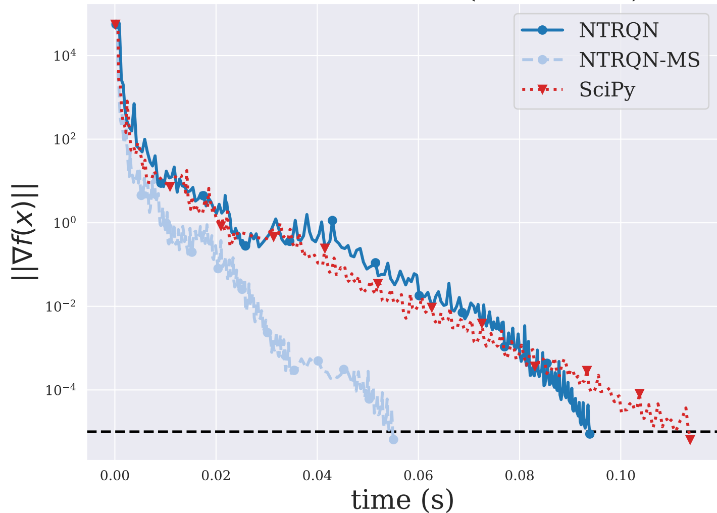
LUKSAN17LS ( n = 100 )
