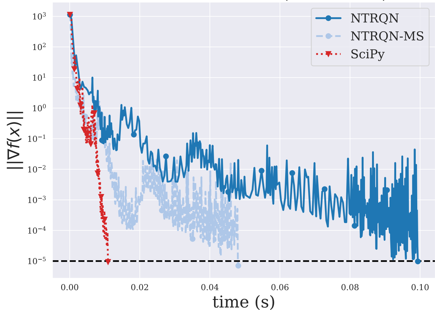
LUKSAN22LS ( n = 100 )
