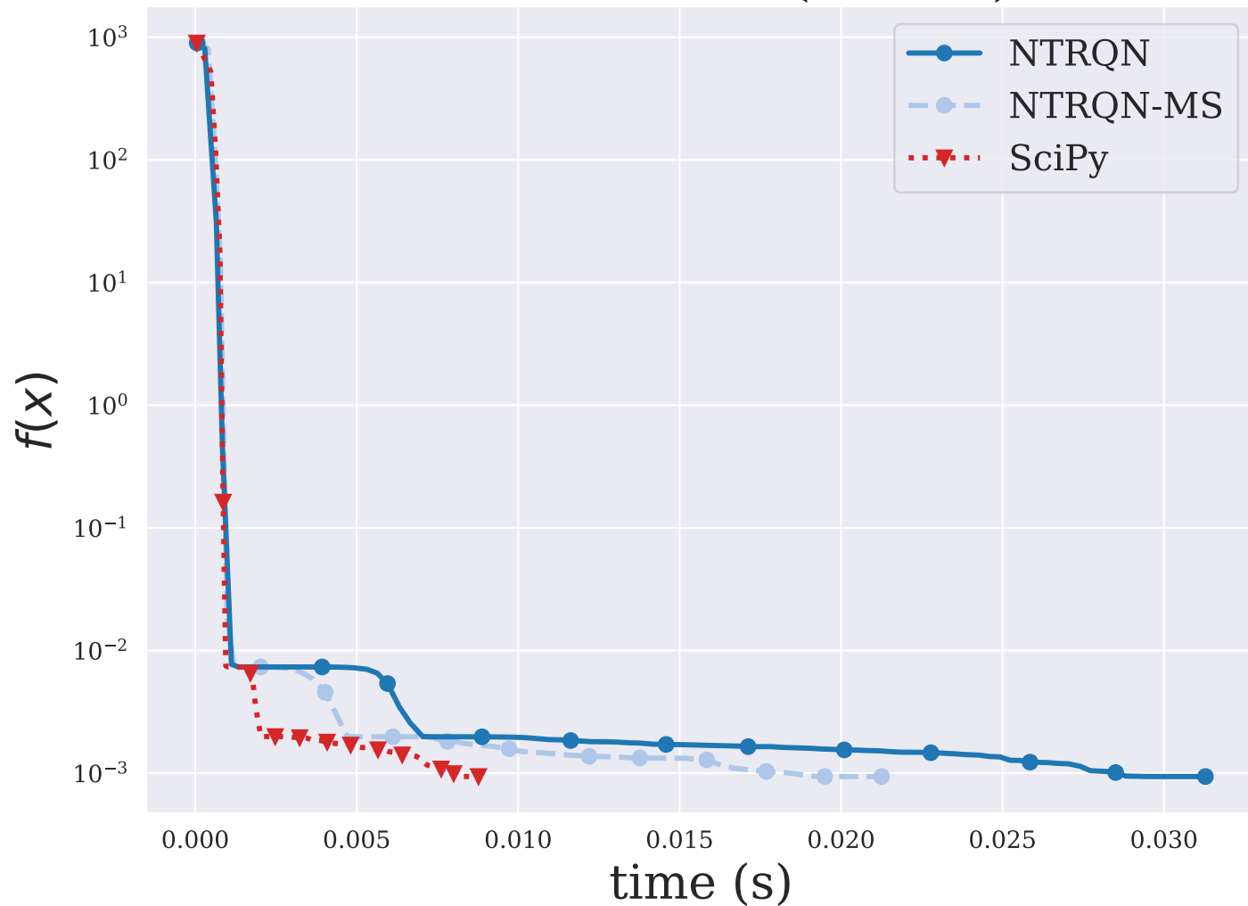
MGH09LS ( n = 4 )
