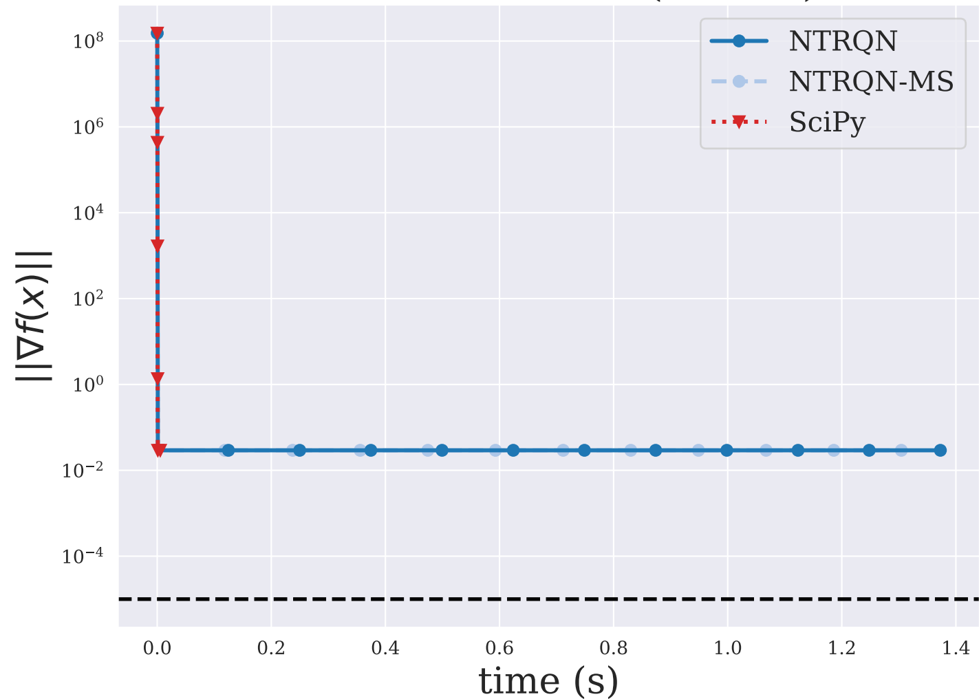
MISRA1DLS ( n = 2 )
