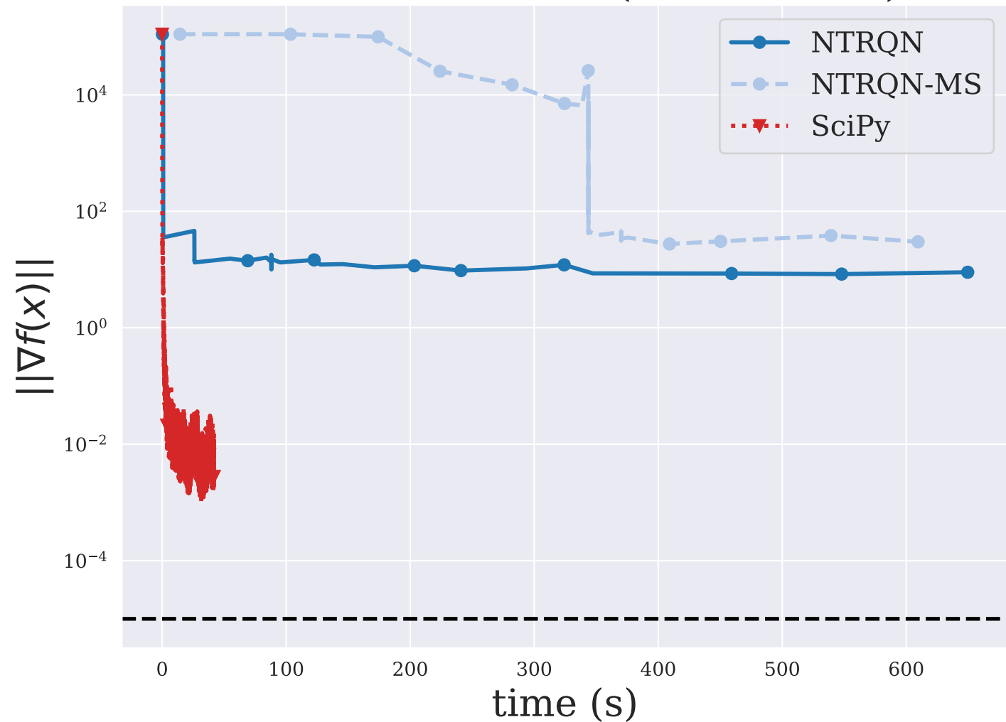
NONCVXUN ( n = 5000 )
