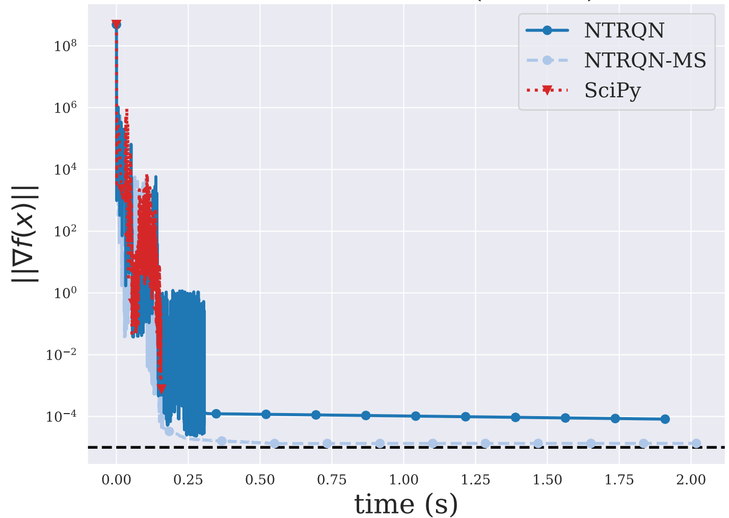
PALMER1C ( n = 8 )
