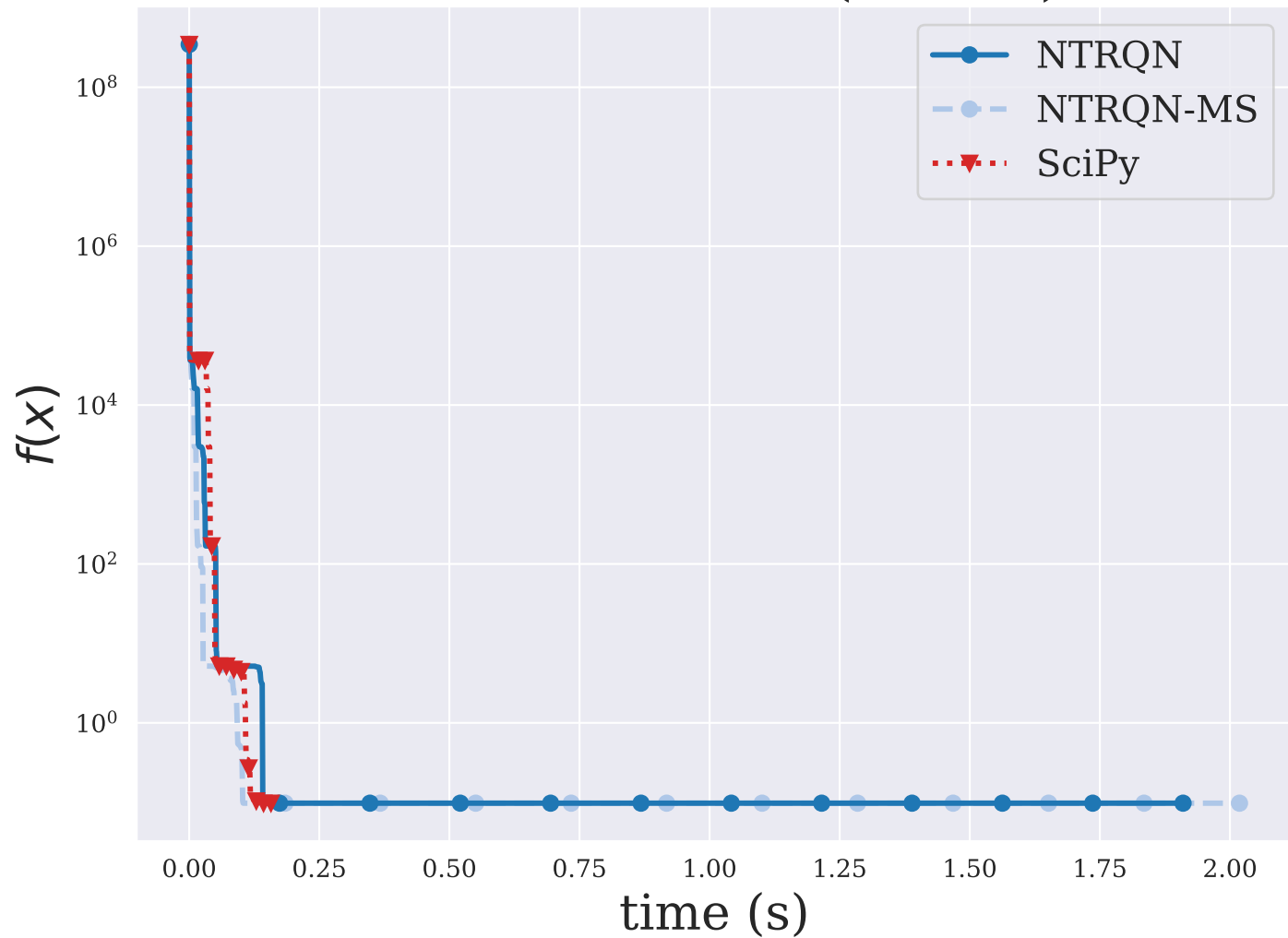
PALMER1C ( n = 8 )
