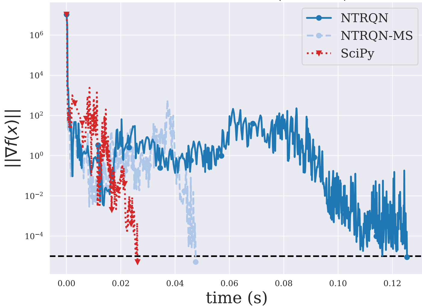
PALMER4C ( n = 8 )
