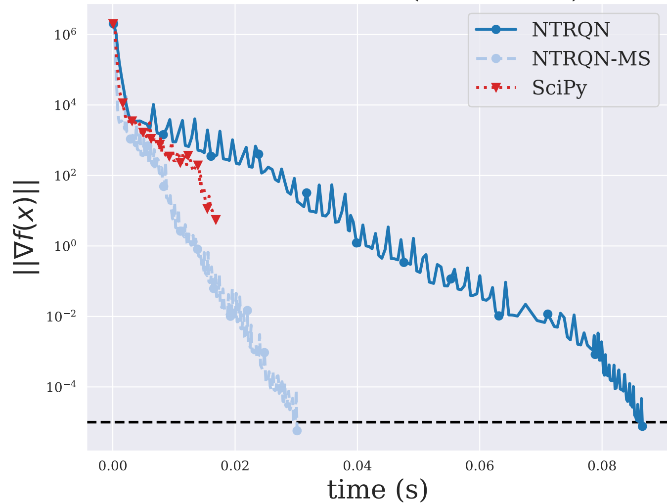
PENALTY2 ( n = 200 )
