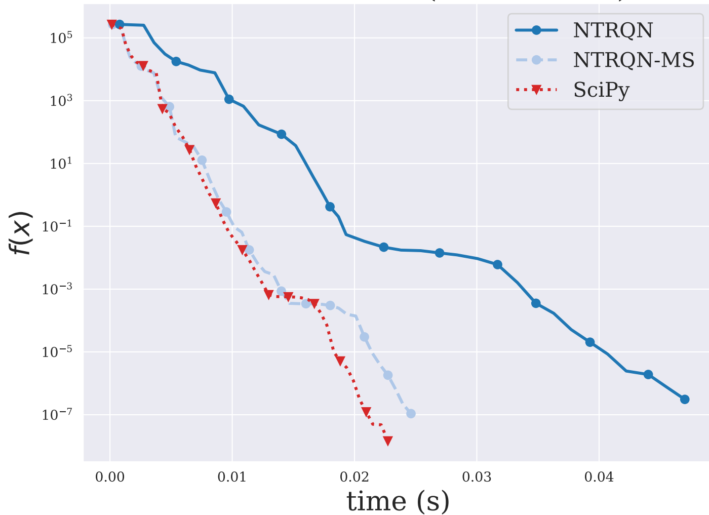
POWELLSG ( n = 5000 )
