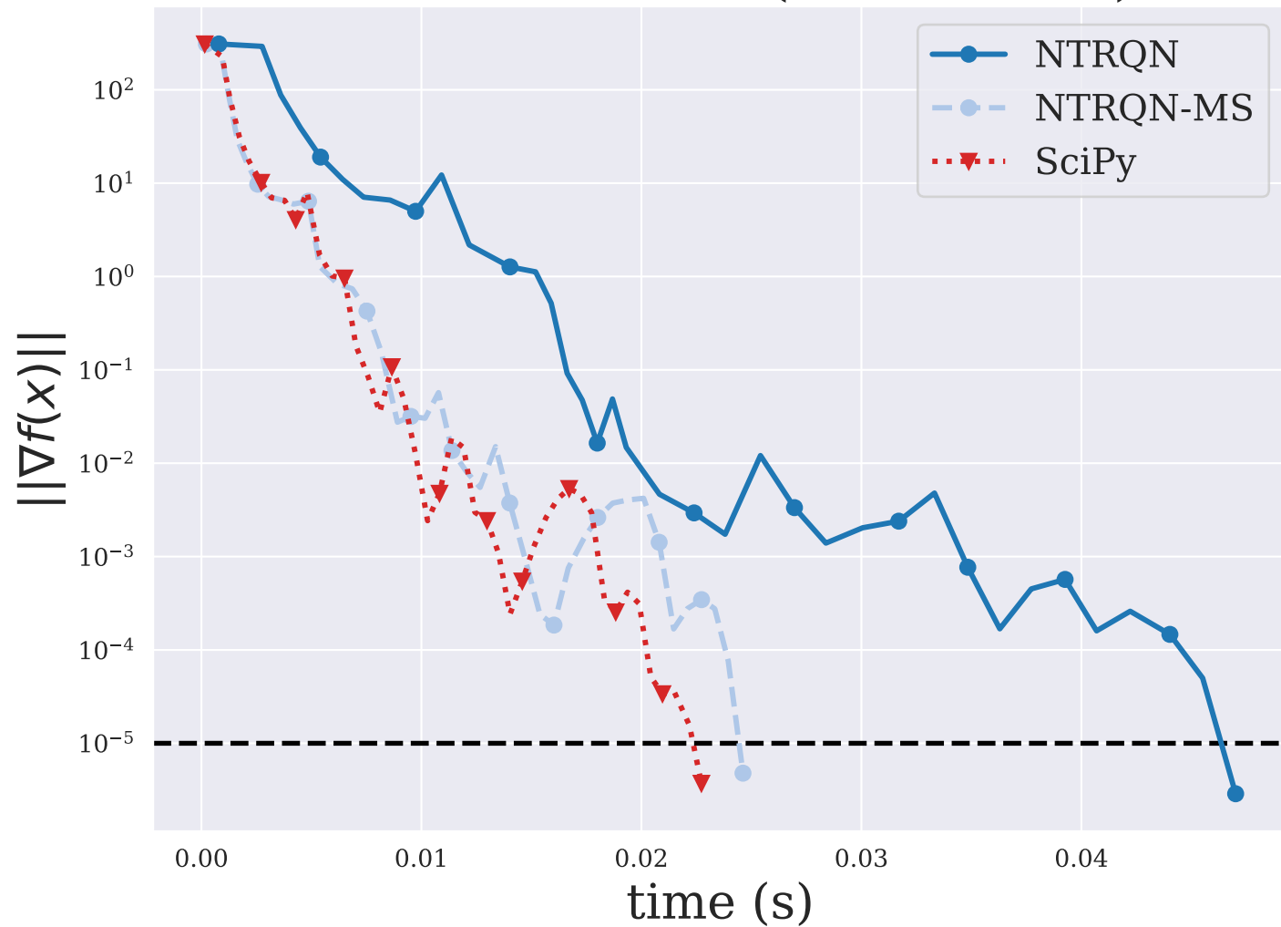
POWELLSG ( n = 5000 )
