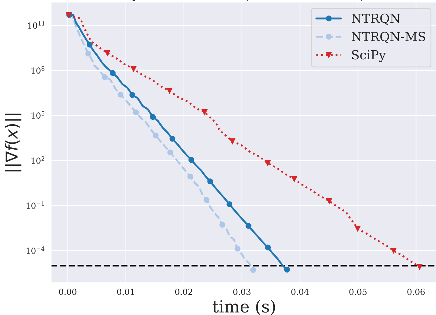
QUARTC ( n = 5000 )
