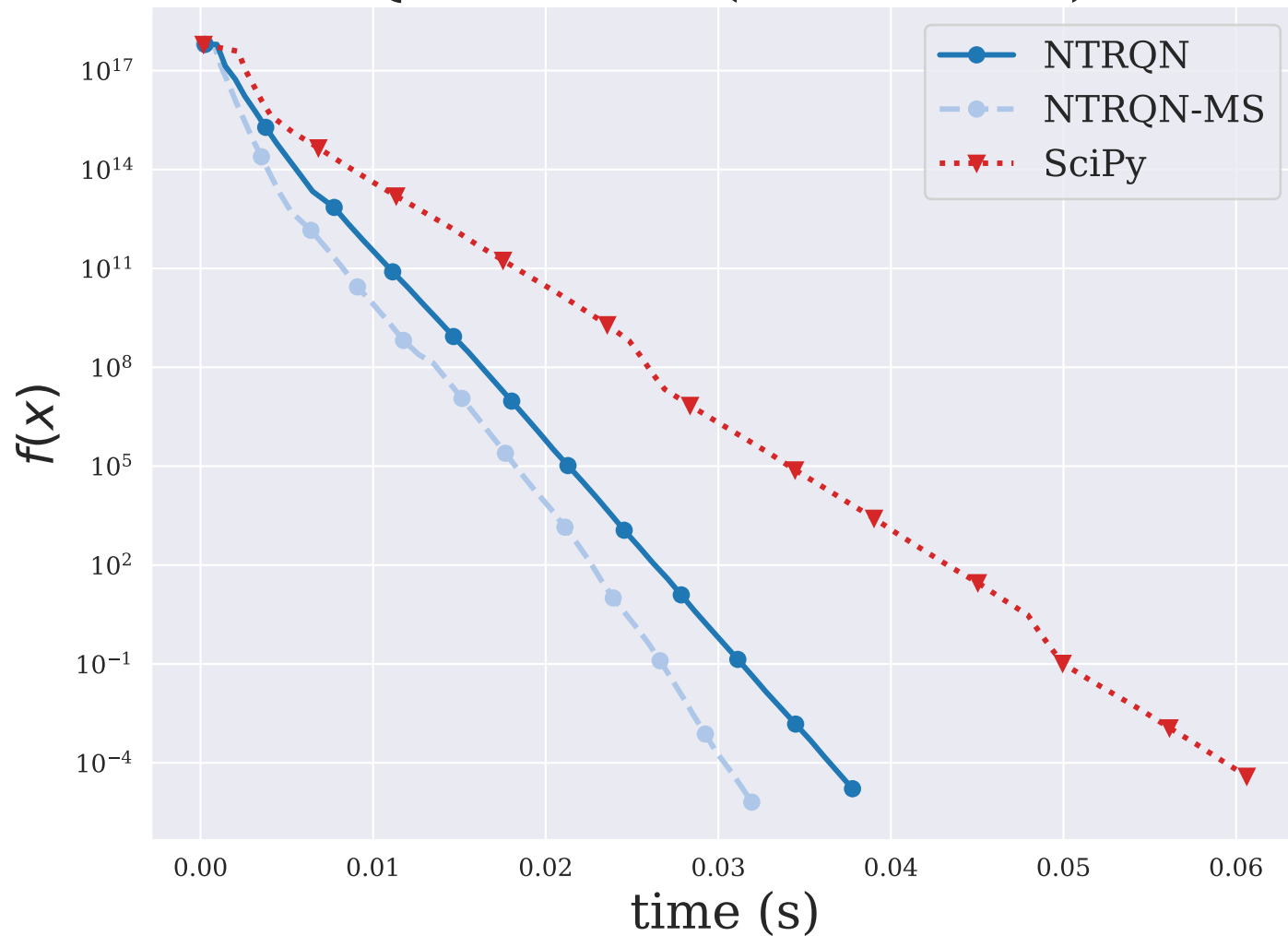
QUARTC ( n = 5000 )
