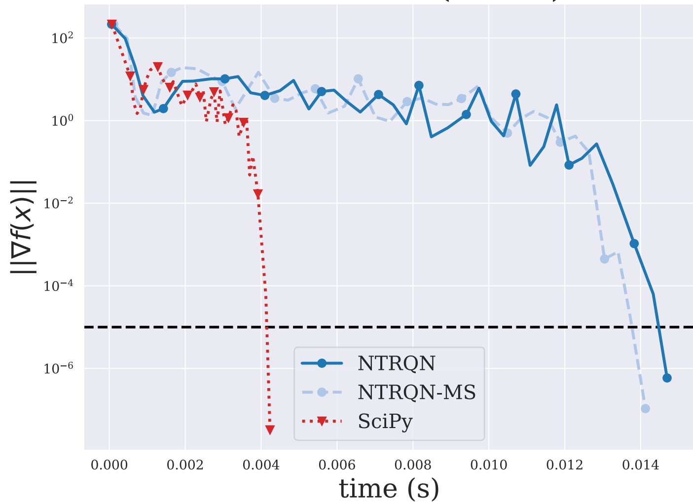
ROSENBUR ( n = 2 )
