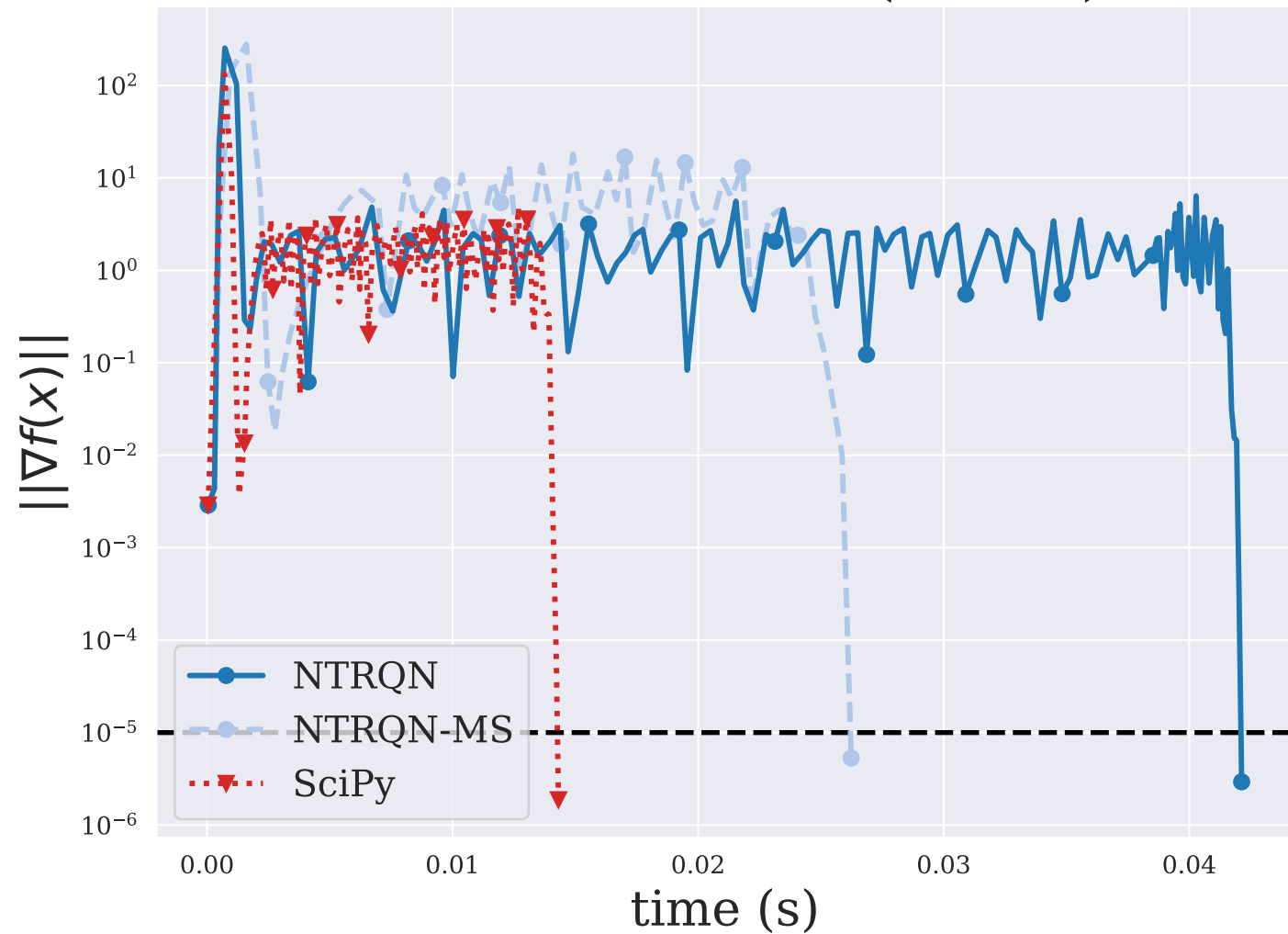
ROSENBRTU ( n = 2 )
