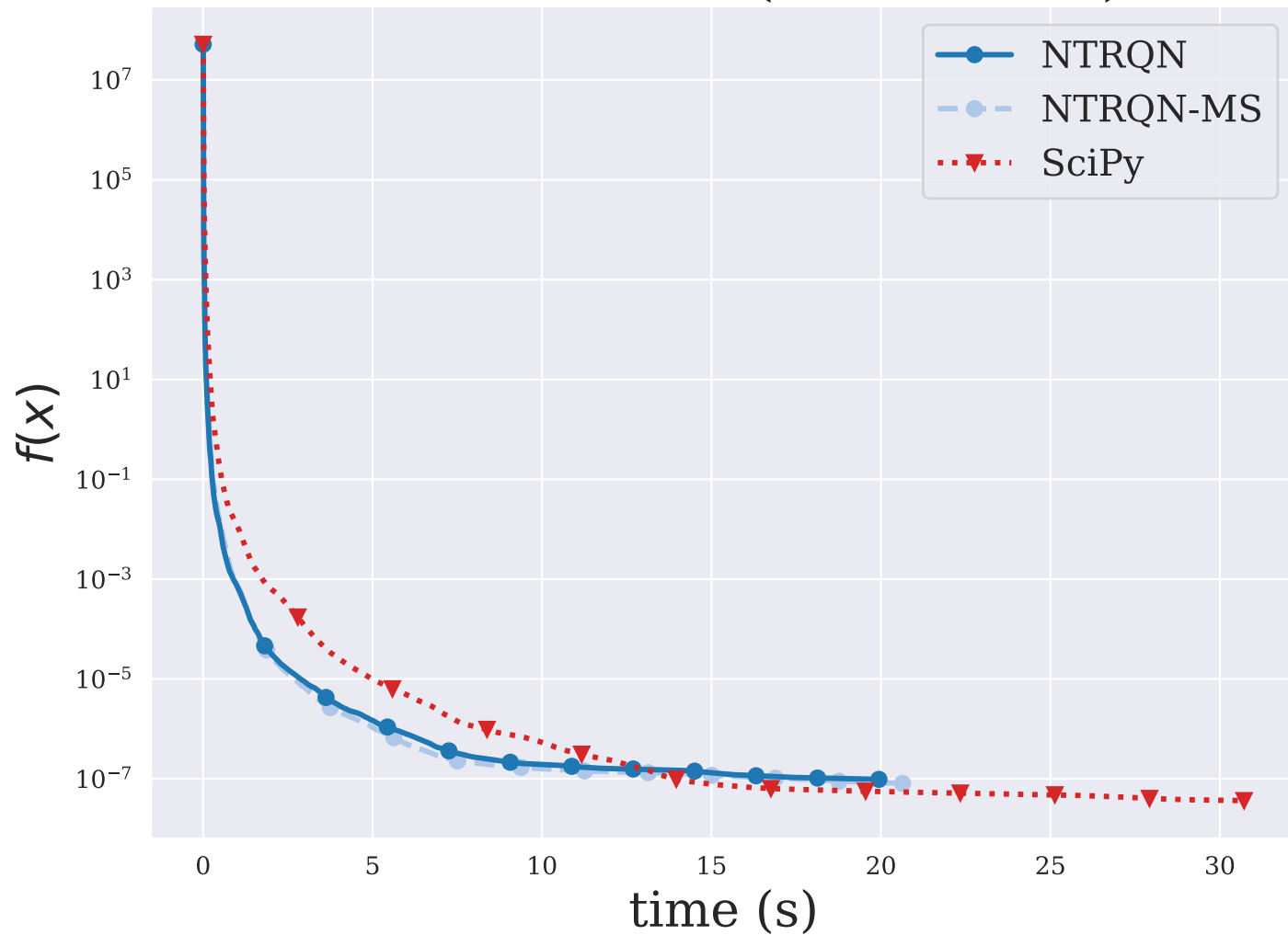
SPARSINE ( n = 5000 )
