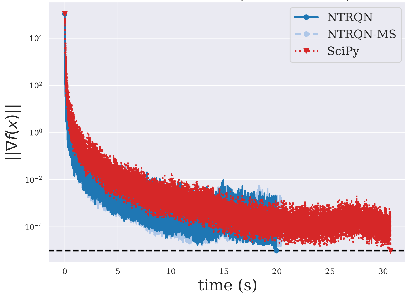
SPARSINE ( n = 5000 )
