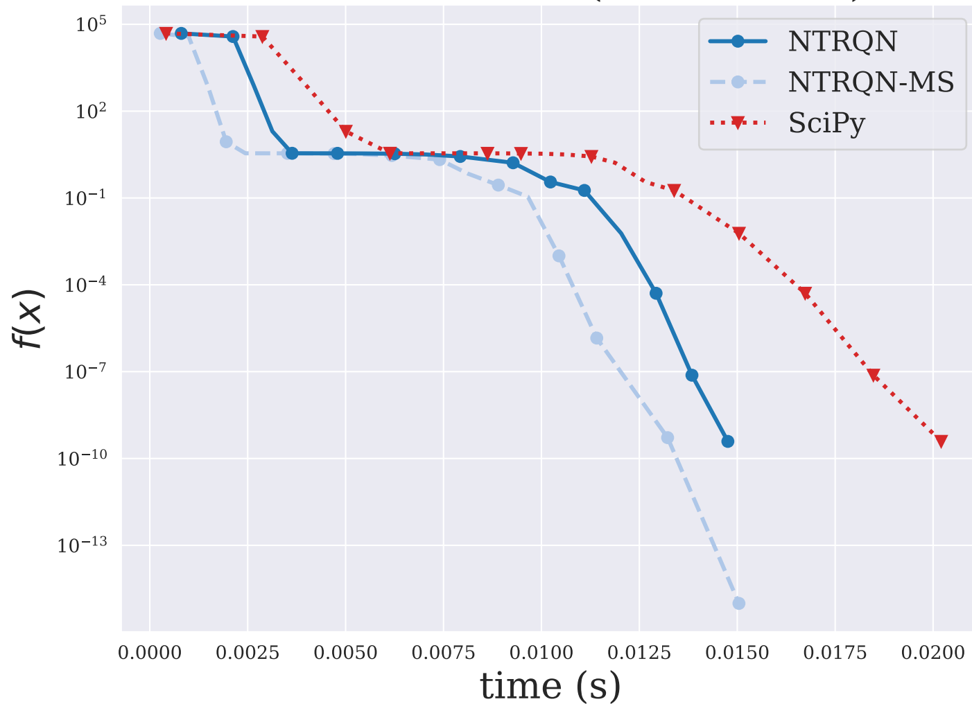
SROSENBR ( n = 5000 )
