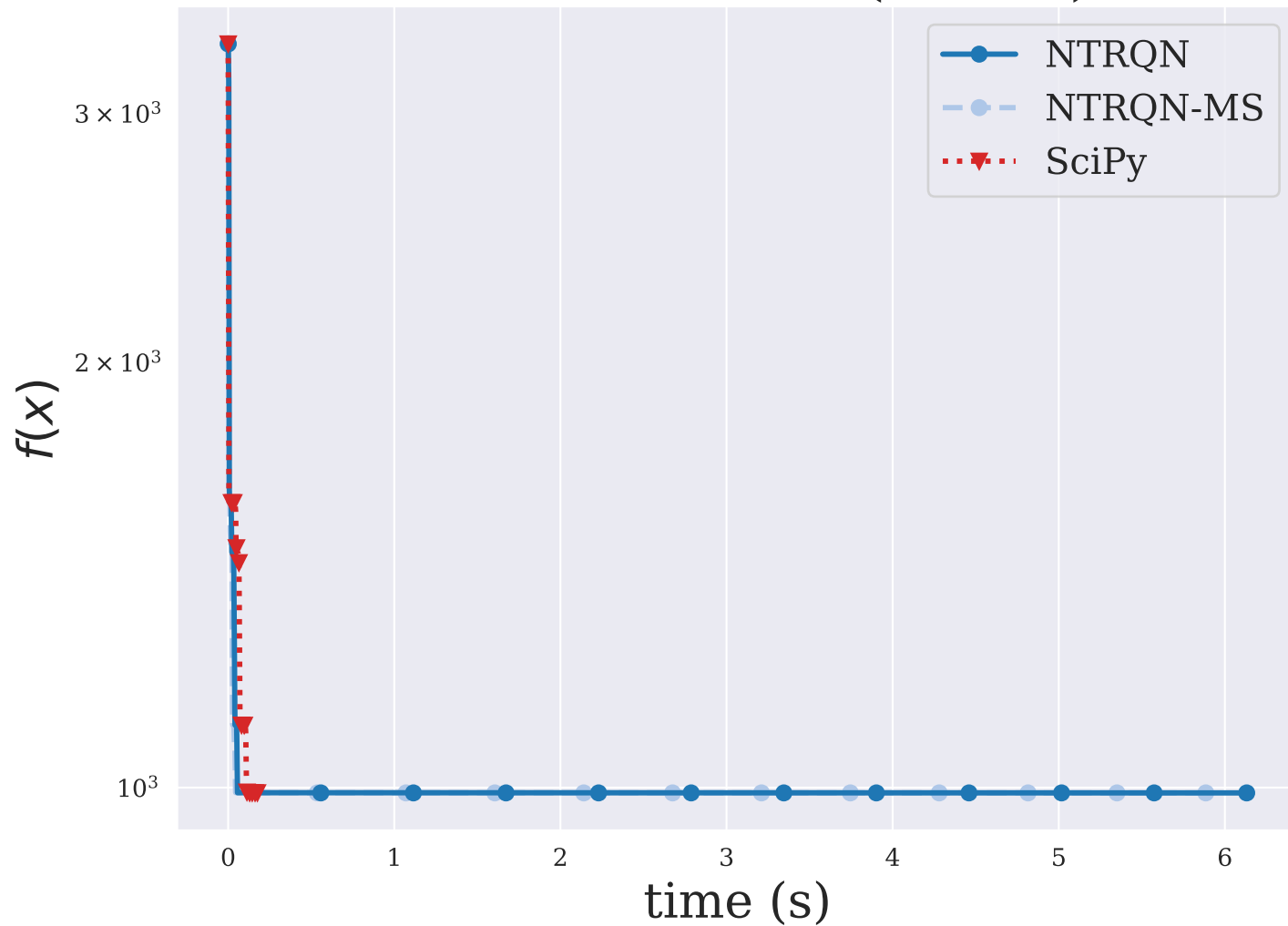
VESUVIOLS ( n = 8 )
