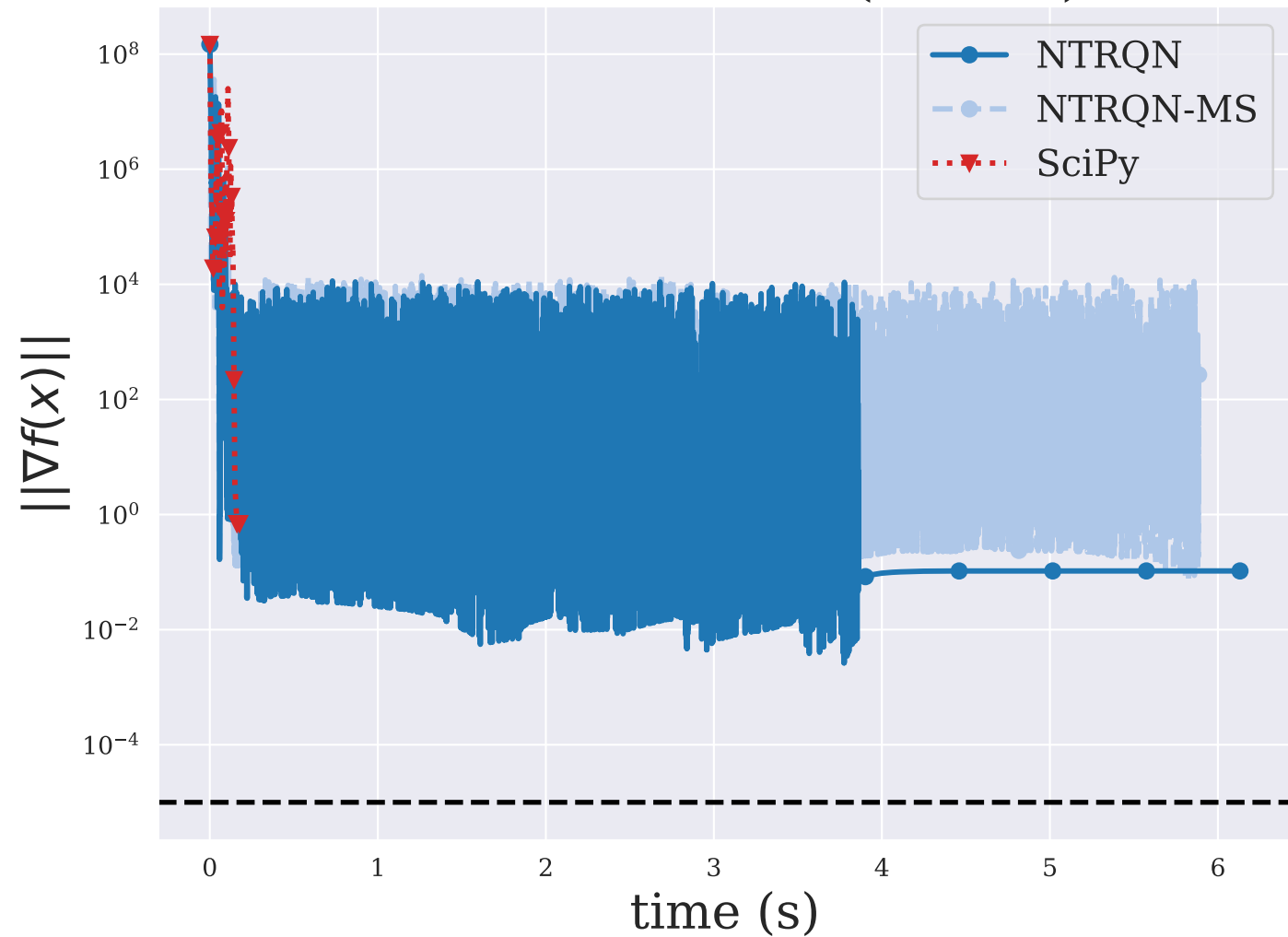
VESUVIOLS ( n = 8 )
