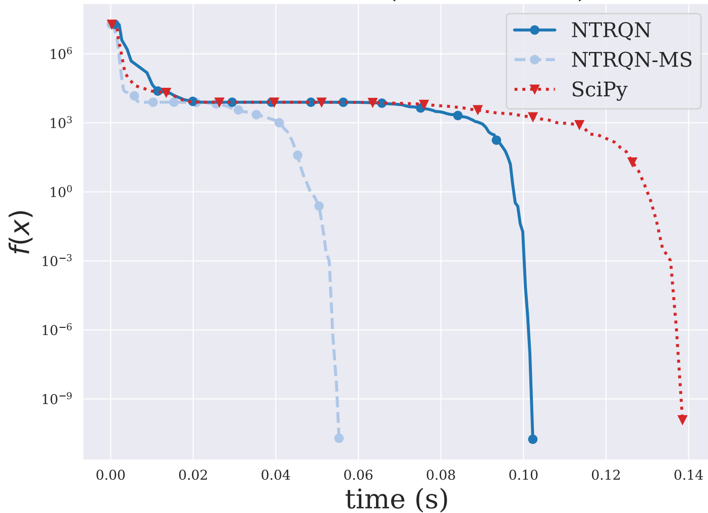
WOODS ( n = 4000 )
