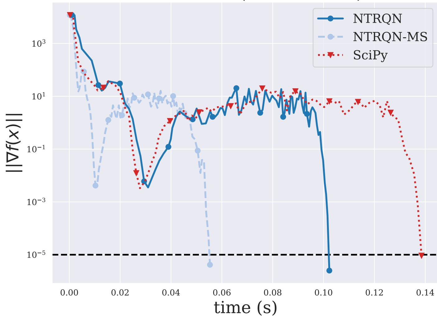
WOODS ( n = 4000 )
