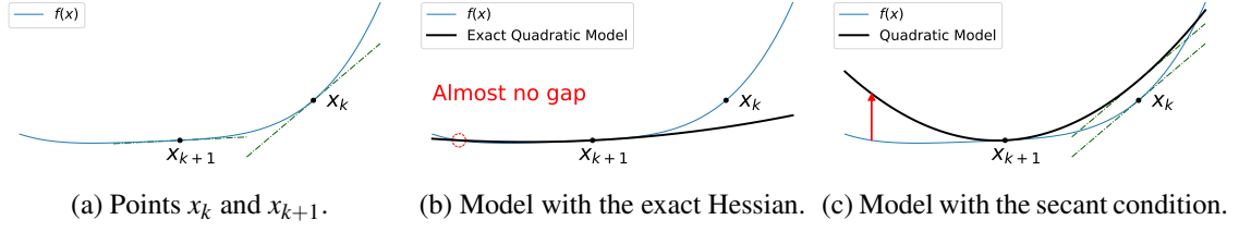
Fig. 2.3: Limitations of the standard secant condition. (a) Function values and gradients at x_k and x_{k+1} are already known. (b) The ideal quadratic model constructed from the exact Hessian fits well around the new point x_{k+1} . (c) The standard secant update may fail to capture curvature adequately.
