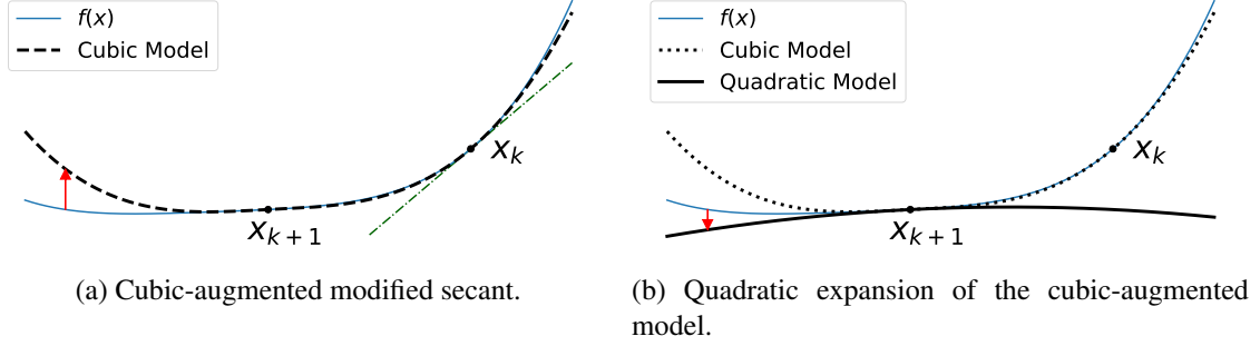
Fig. 2.6: Cubic-augmented modified secant equation. In Figure 2.6a, by incorporating a cubic term \eta \|x - x_k\|^3 in the model, the modified secant equation B_k^C s_k = y_k + \sigma_k^C s_k enables simultaneous satisfaction of both conditions at the previous point. In Figure 2.6b, while the cubic model satisfies both function value and gradient conditions, its underlying quadratic component may be indefinite or negative definite.
