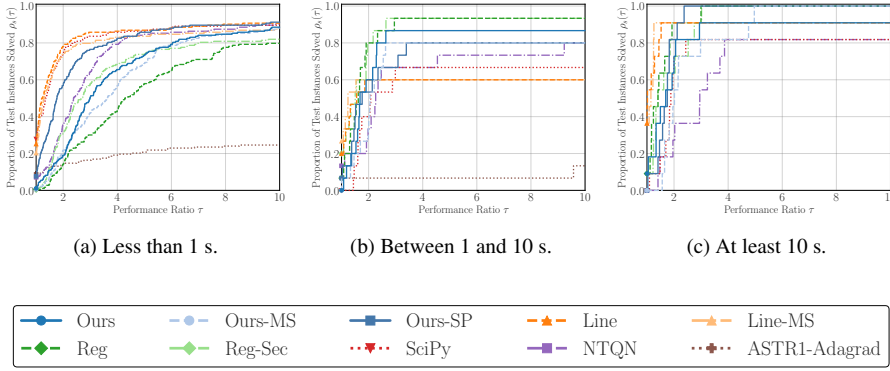
Fig. 6: Performance profiles for the 64-bit setting at \epsilon_{\text{gtol}} = 10^{-3} , grouped by the best runtime attained by any method on each problem instance.
