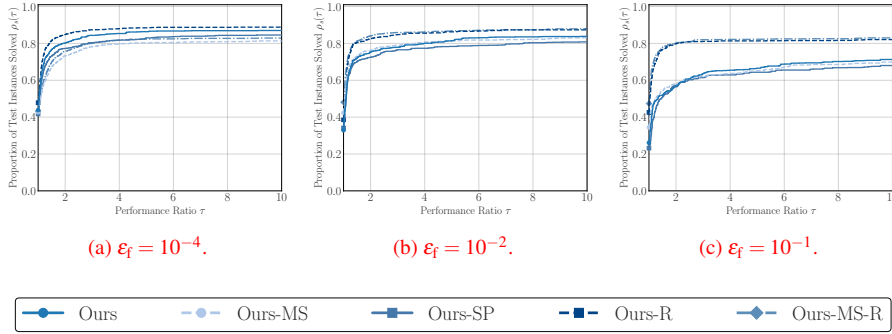
Fig. 2: Performance profile for the deliberately adverse joint function-and-gradient noise setting (componentwise level 10^{-3} ) and \epsilon_{\text{gtol}} = 10^{-2} . This experiment lies outside the exact-gradient theory.
