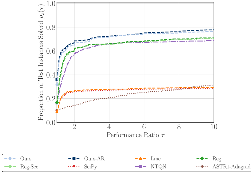
Fig. 2: Performance profile for the joint function-and-gradient noise setting (componentwise level 10^{-3} ) and \epsilon_{\text{gtol}} = 10^{-2} .
