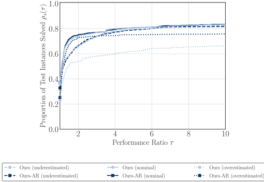
Fig. 3: Performance profiles for error-bound misspecification under function-value-only noise of level 10^{-3} and \varepsilon_{\text{tol}} = 10^{-2} .
