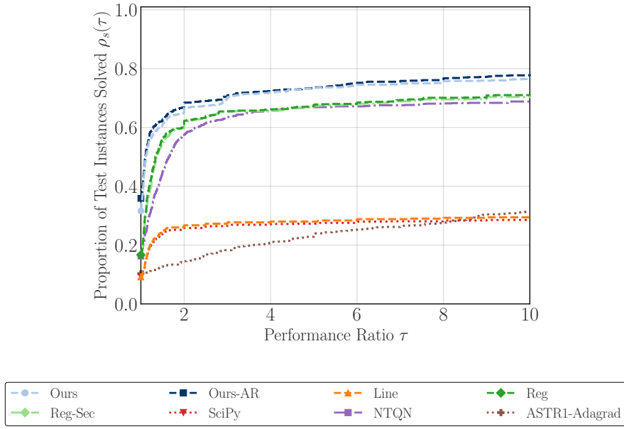
Fig. 2: Performance profile for the deliberately adverse joint function-and-gradient noise setting (componentwise level 10^{-3} ) and \epsilon_{\text{gtol}} = 10^{-2} .
