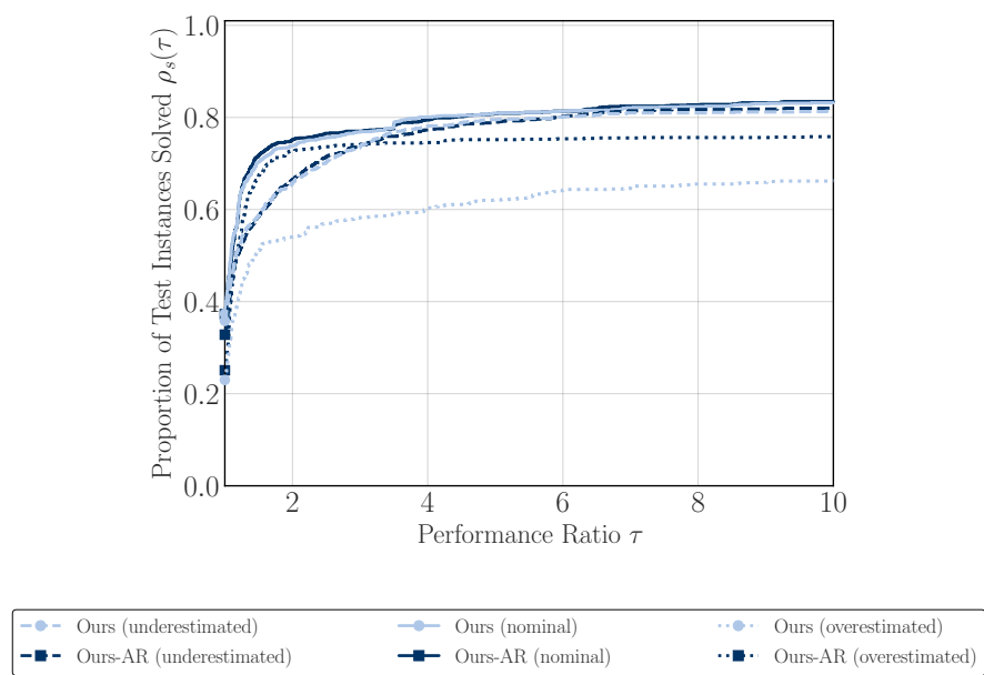
Fig. 3: Performance profiles for error-bound misspecification under function-value-only noise of level 10^{-3} and \varepsilon_{\text{gtol}} = 10^{-2} .
