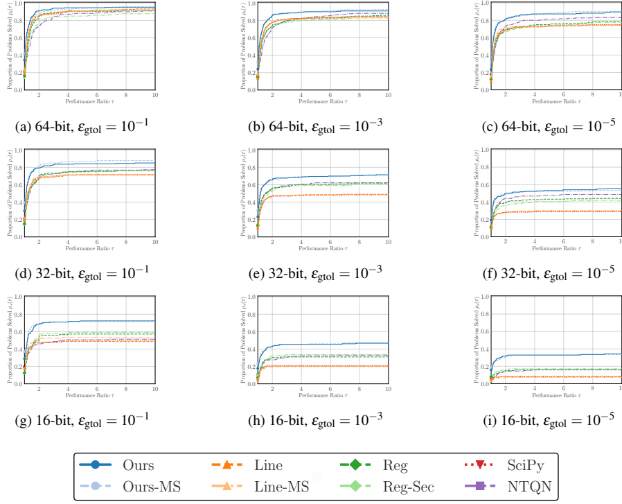
Fig. 2: Performance profiles across different floating-point precisions (64-, 32-, and 16-bit) and tolerance levels. The results demonstrate the robustness of the proposed methods.
