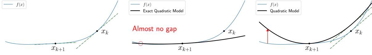
Figure 13: Limitations of the standard secant condition. (a) Function values and gradients at x_k and x_{k+1} are already known. (b) The ideal quadratic model constructed from the exact Hessian fits well around the new point x_{k+1} . (c) The standard secant condition may fail to capture curvature adequately.
