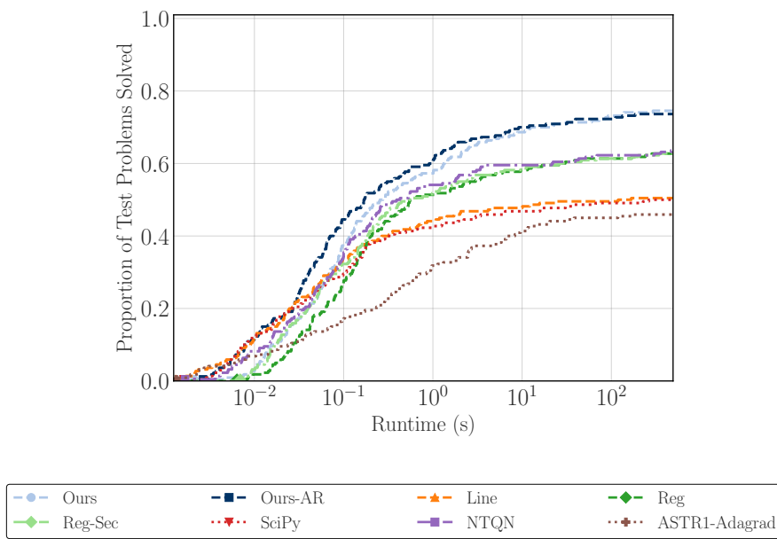
Fig. 6: Proportion of 32-bit test problems attaining \varepsilon_{\text{gtol}} = 10^{-3} as a function of runtime.
