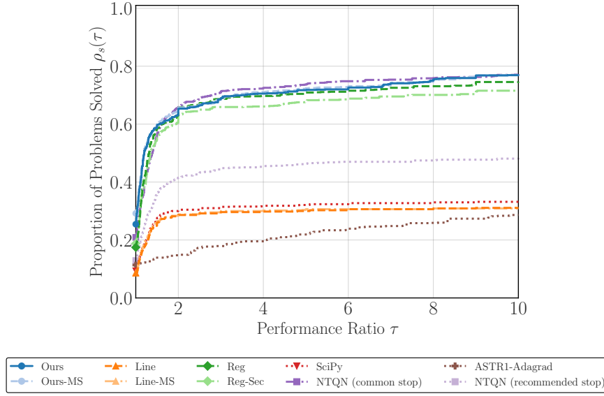
Fig. 1: Theory-aligned function-value-noise results at noise level 10^{-3} , supplied error bound \varepsilon_f = 10^{-2} , and \varepsilon_{\text{gtol}} = 10^{-2} .
