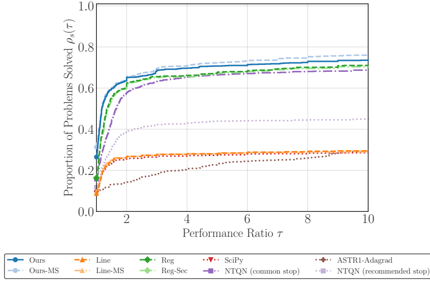
Fig. 2: Performance profile for the deliberately adverse joint function-and-gradient noise setting (componentwise level 10^{-3} ) and \epsilon_{\text{gtol}} = 10^{-2} ; this experiment lies outside the exact-gradient theory.
