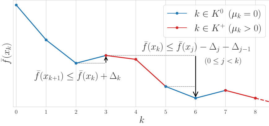
Fig. 1: An example of the sequence \{\bar{f}(x_k)\} generated by Algorithm 1. Each iteration index k is classified into K^0 (blue) or K^+ (red). The relaxed Armijo condition eq. (5) ensures a temporary increase of \bar{f} is at most \Delta_k , such as from k = 2 to k = 3 . We only set \mu_k = 0 when the sufficient decrease condition eq. (7) is satisfied over iterations in K^0 , such as at k = 6 , preventing unbounded growth or oscillation of \bar{f} .
