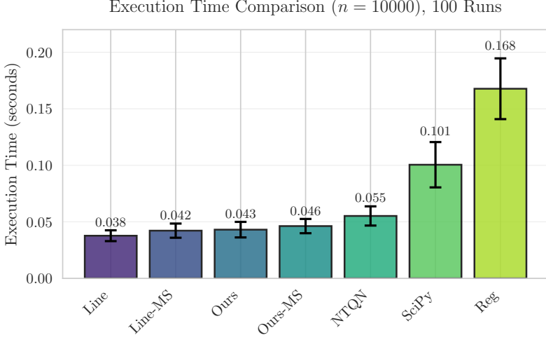
Fig. 4: Mean execution times for the experiment in section 6.3. This plot roughly indicates the extra computational overhead of each method. Error bars represent one standard deviation over 100 runs.
