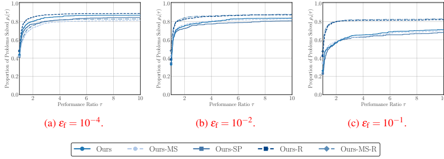
Fig. 3: Performance profiles for error-bound misspecification under function-value-only noise of level 10^{-3} and \varepsilon_{\text{gtol}} = 10^{-2} .
