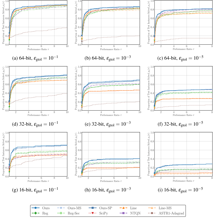
Fig. 4: Performance profiles across floating-point precisions (64-, 32-, and 16-bit) and tolerance levels.
