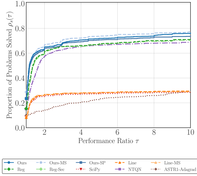
Fig. 2: Performance profile for the deliberately adverse joint function-and-gradient noise setting (componentwise level 10^{-3} ) and \varepsilon_{\text{gtol}} = 10^{-2} . This experiment lies outside the exact-gradient theory.
