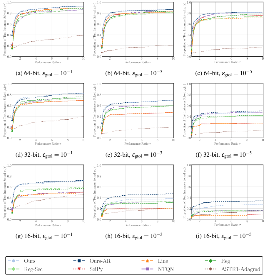
Fig. 4: Performance profiles across floating-point precisions (64-bit, 32-bit, and 16-bit) and tolerance levels.
