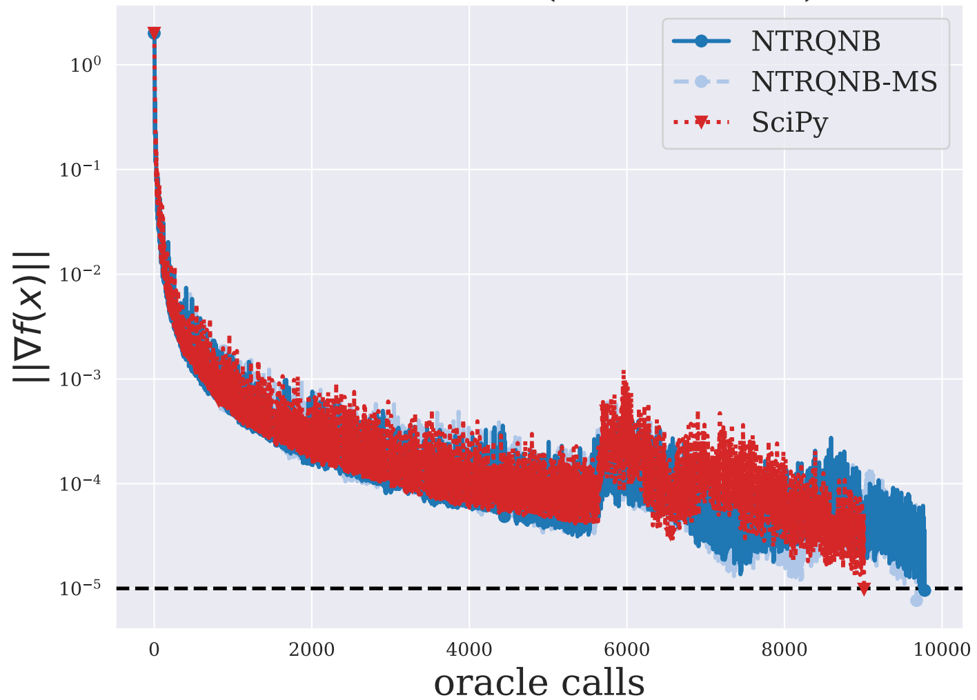
BIGGSB1 ( n = 5000 )
