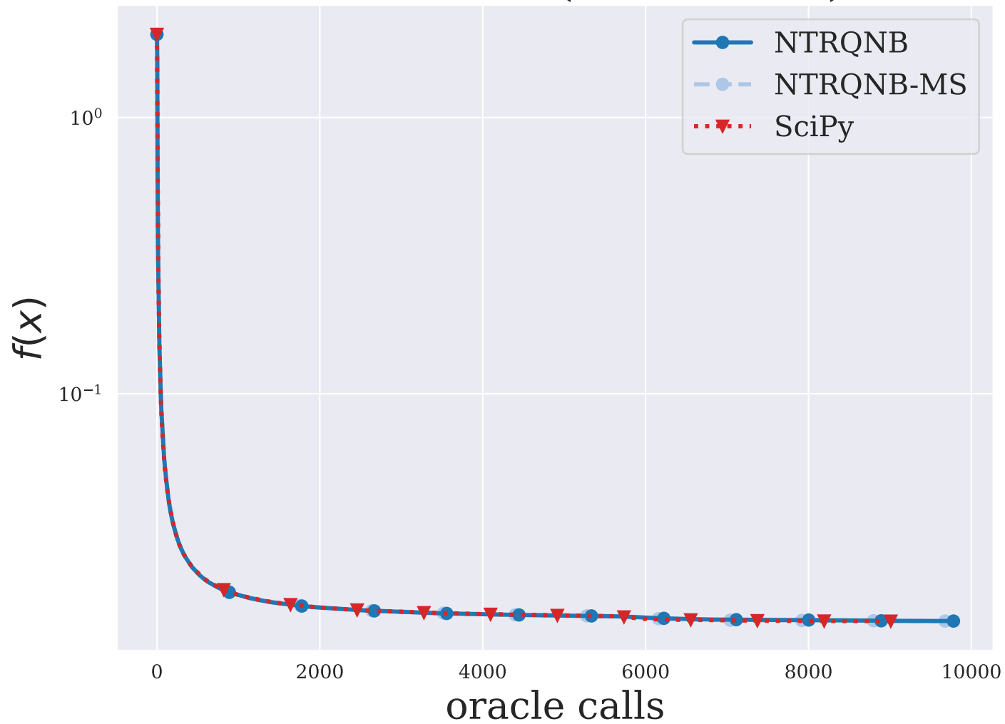
BIGGSB1 ( n = 5000 )
