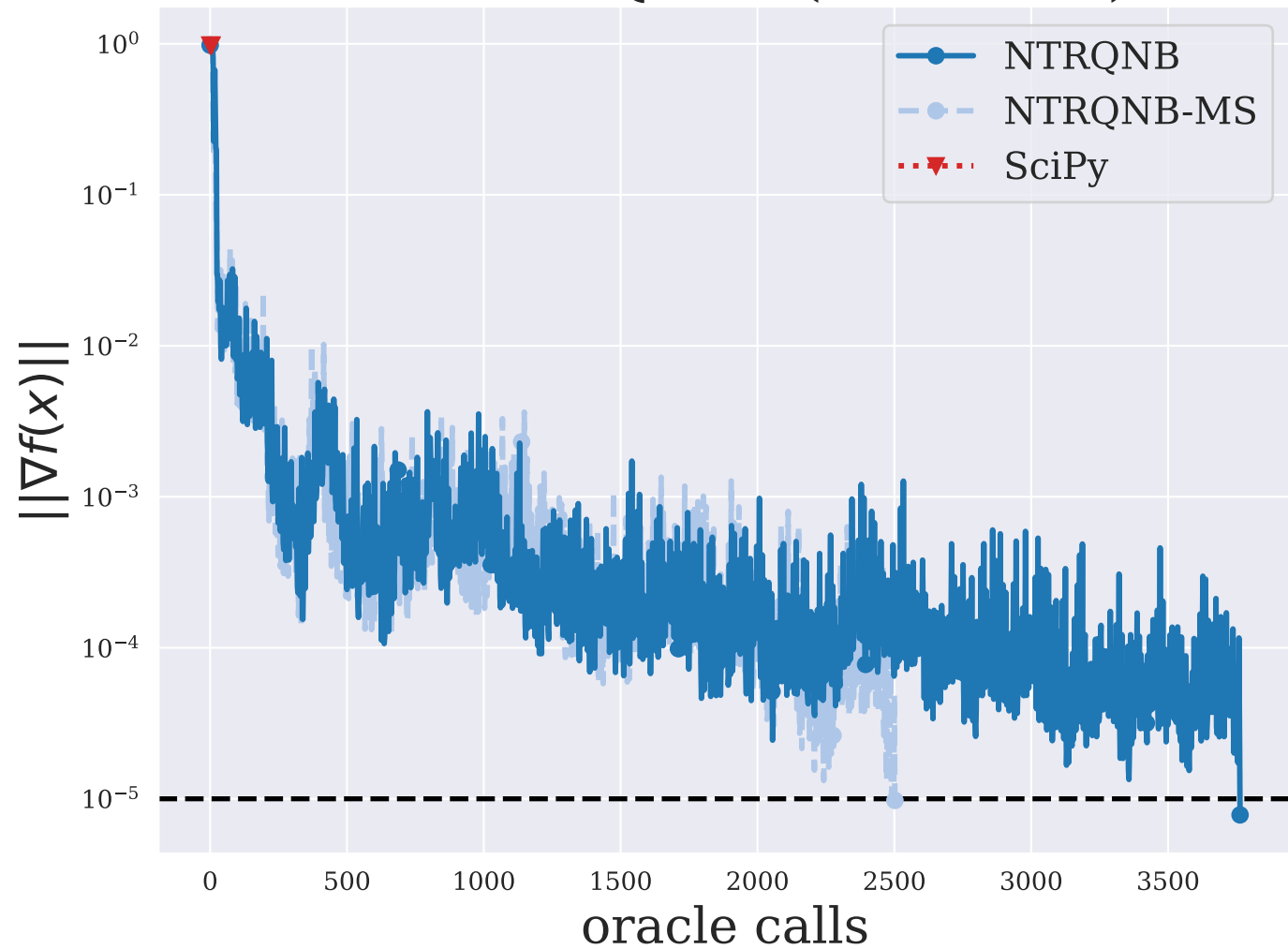
CHEBYQAD ( n = 100 )
