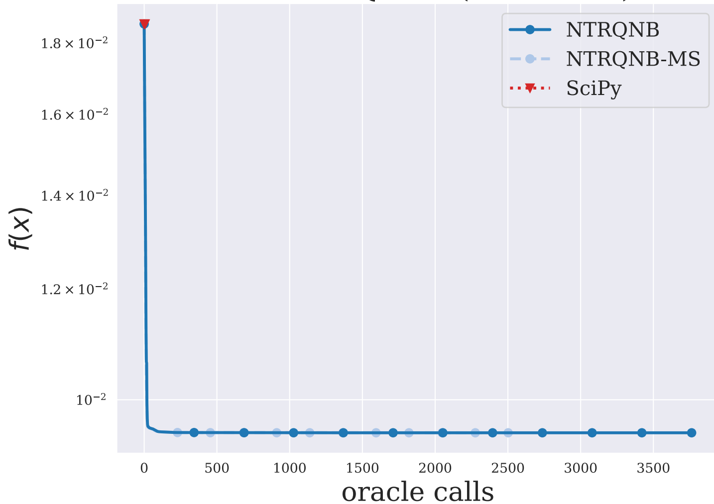
CHEBYQAD ( n = 100 )
