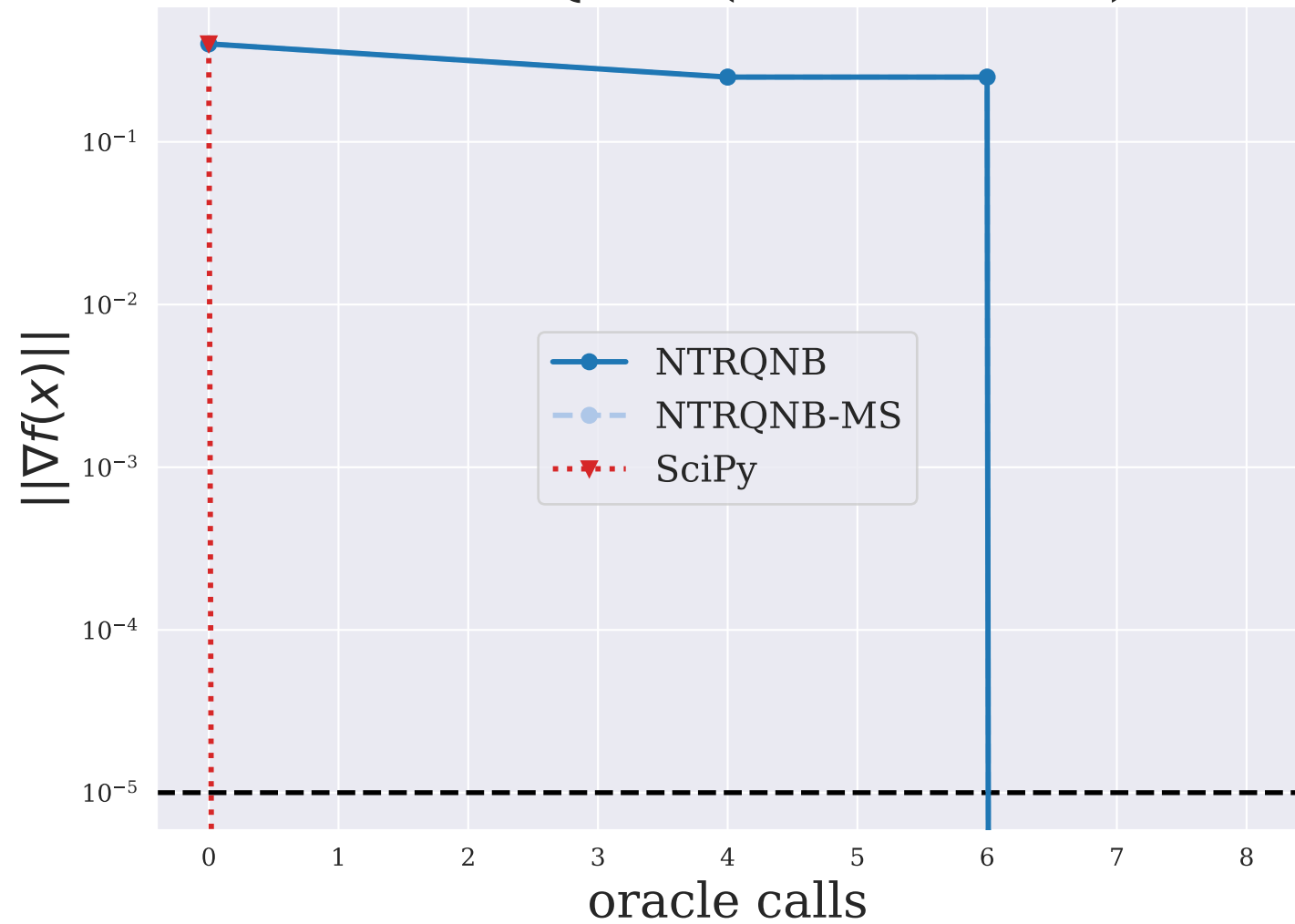
CVXBQP1 ( n = 10000 )
