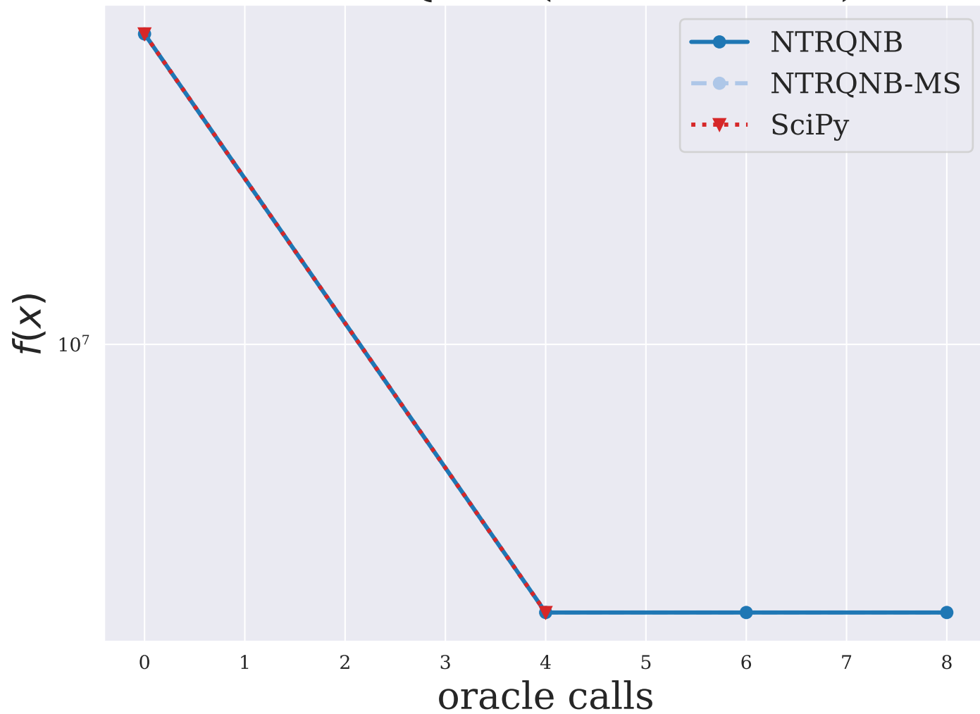
CVXBQP1 ( n = 10000 )
