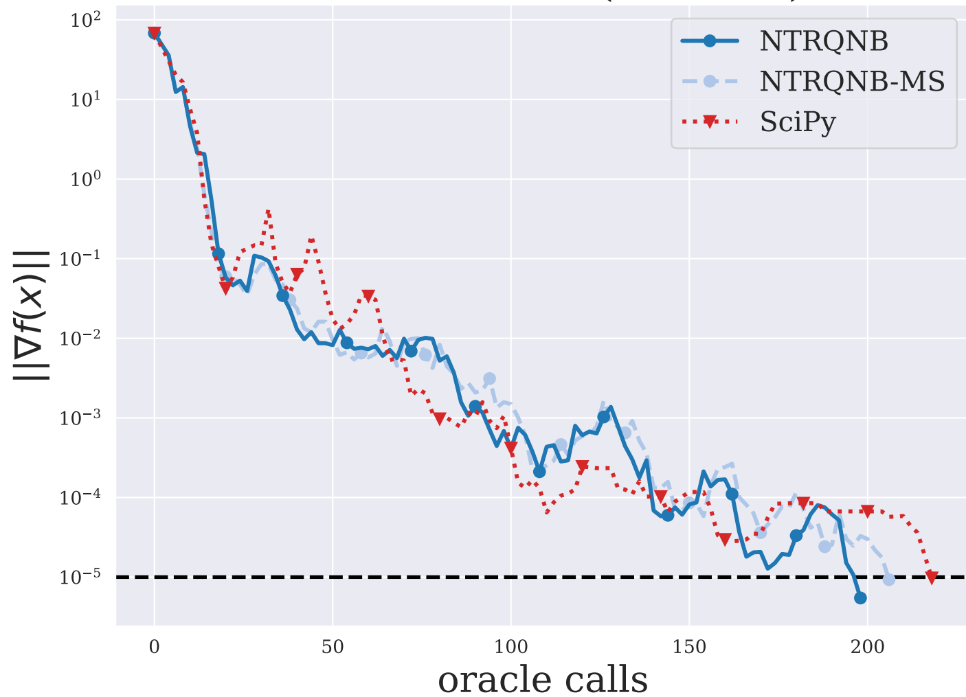
DECONVB ( n = 51 )
