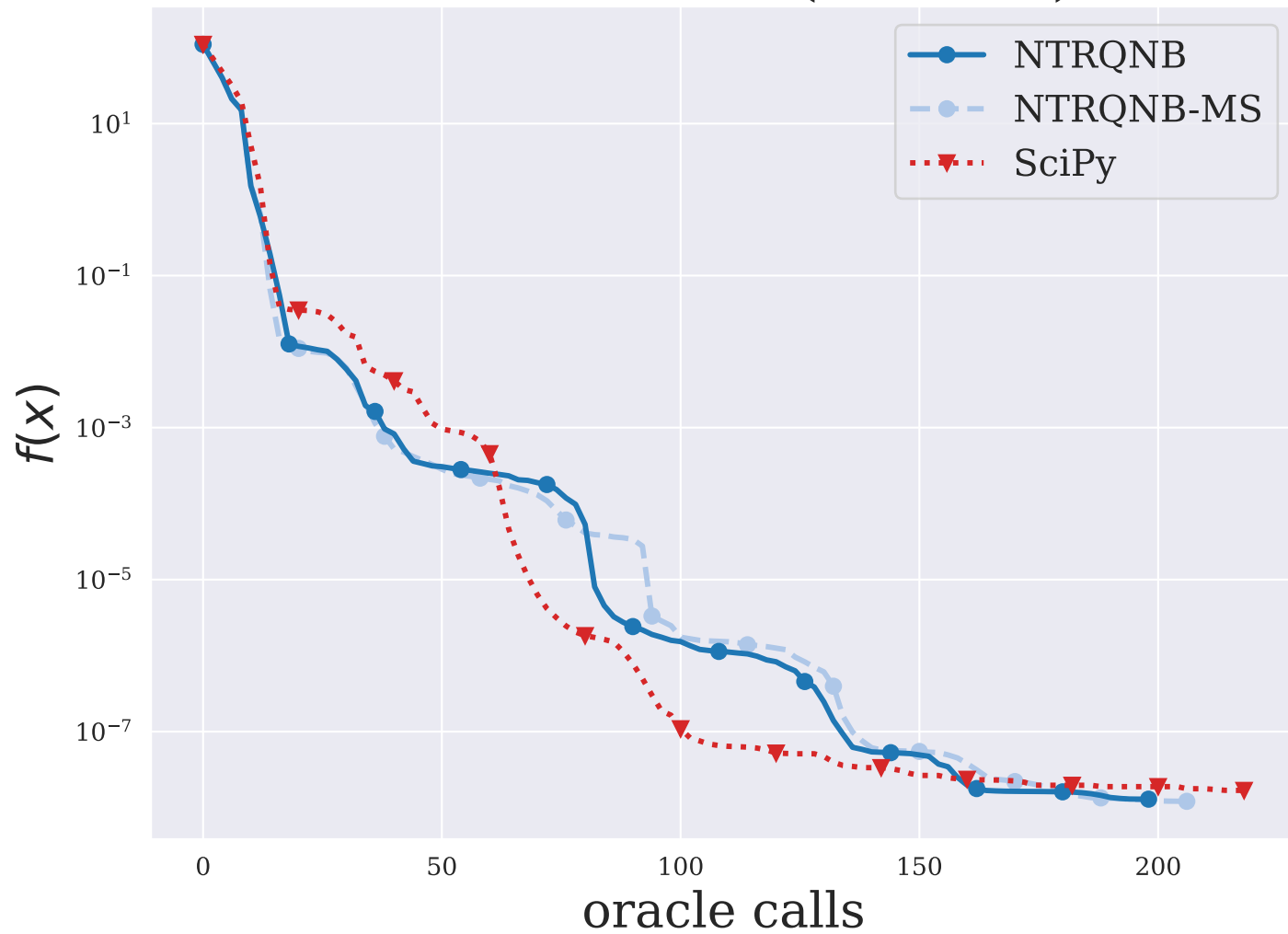
DECONVB ( n = 51 )
