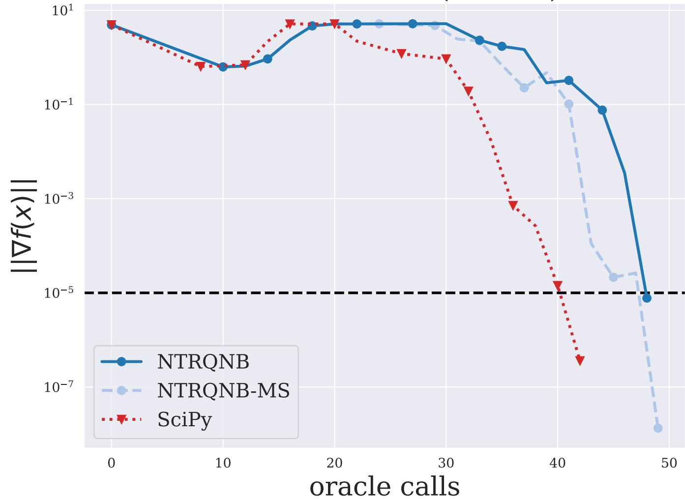
FBRAINLS ( n = 2 )
