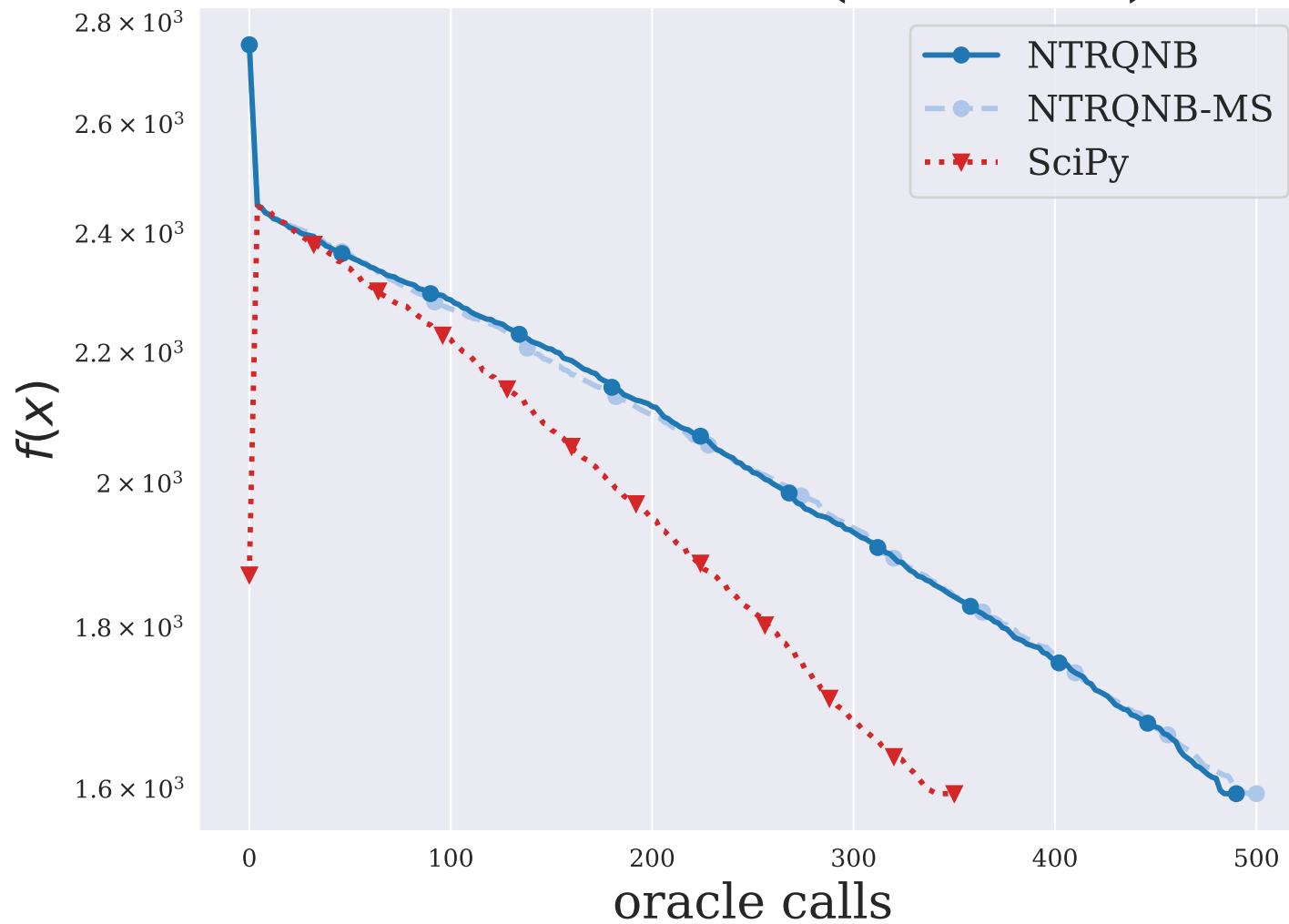
GENROSEB ( n = 500 )
