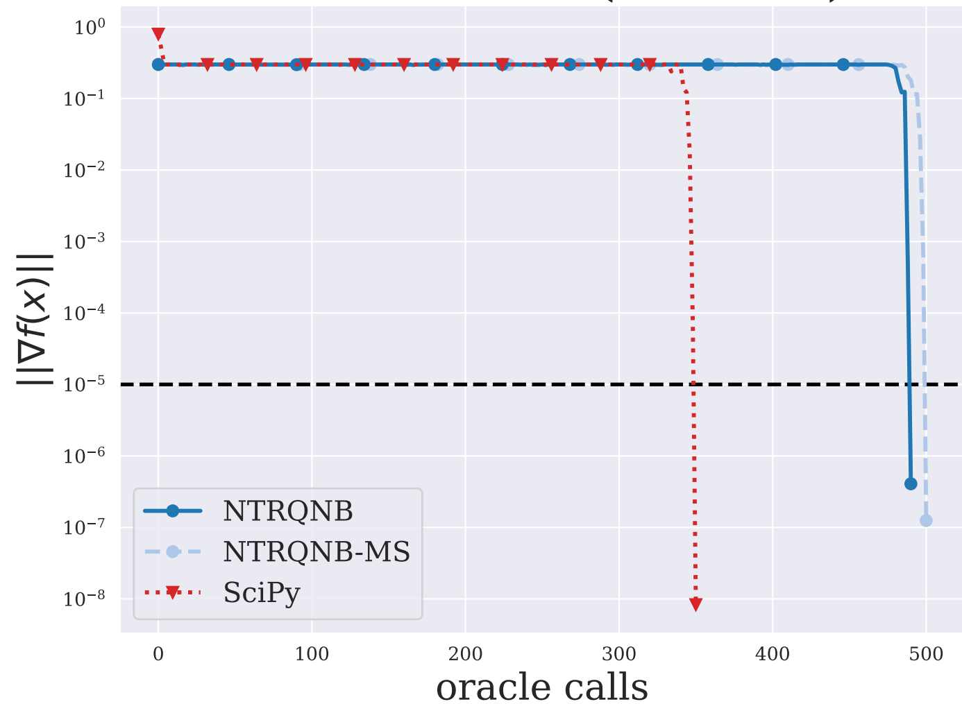
GENROSEB ( n = 500 )
