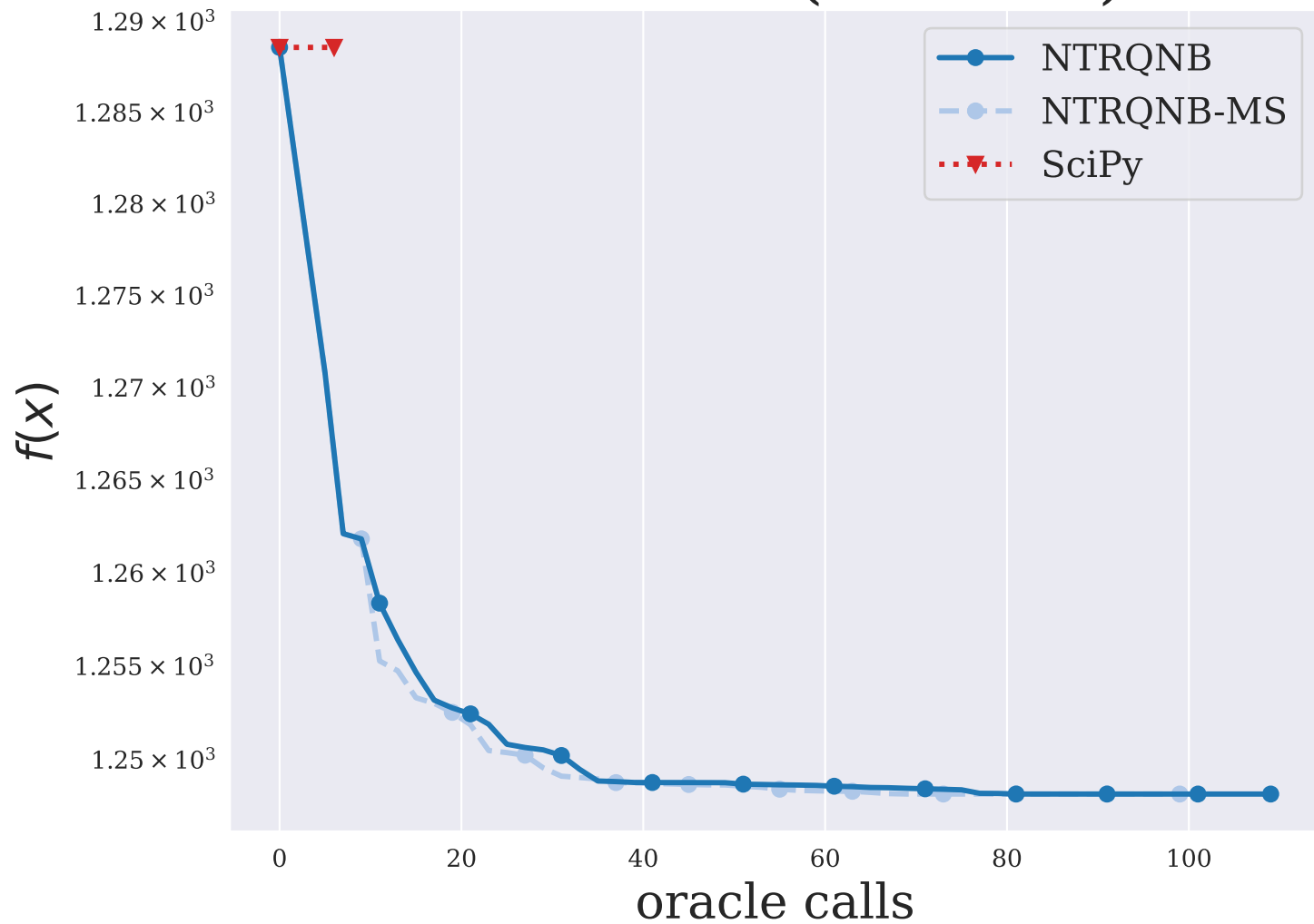
HOLMES ( n = 180 )
