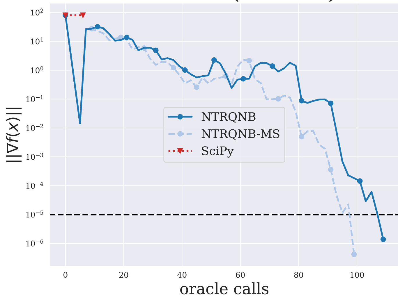
HOLMES ( n = 180 )
