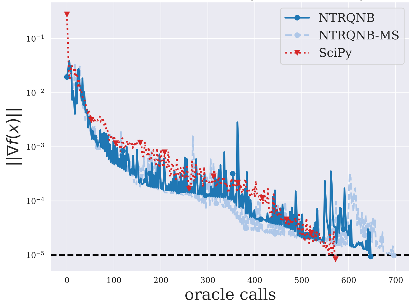
MINSURFO ( n = 5002 )
