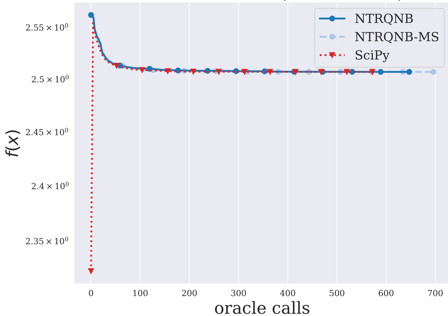
MINSURFO ( n = 5002 )
