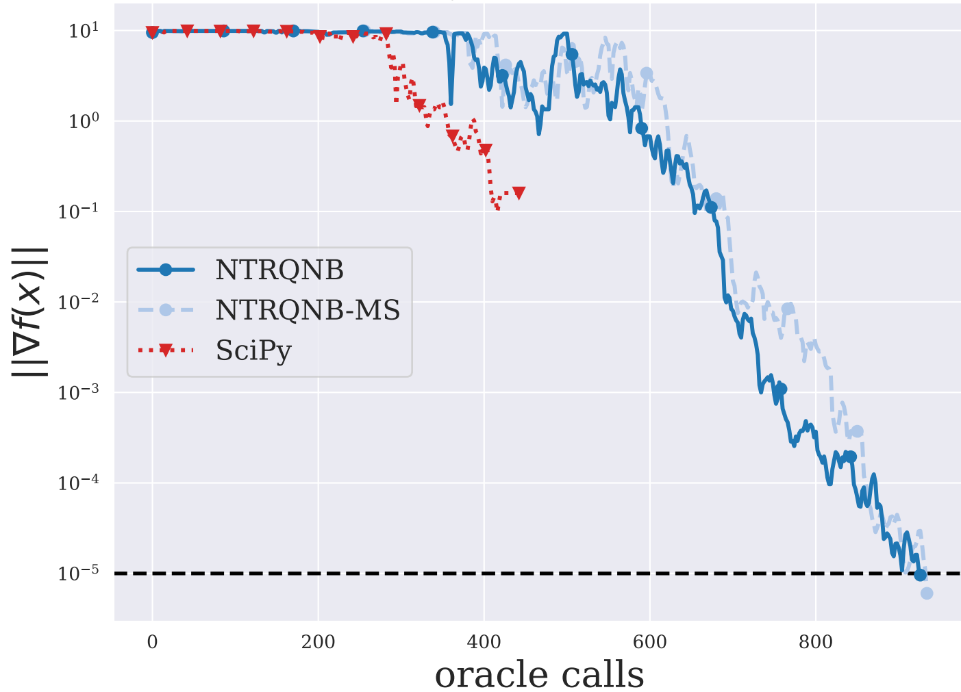
NCVXBQP3 ( n = 10000 )
