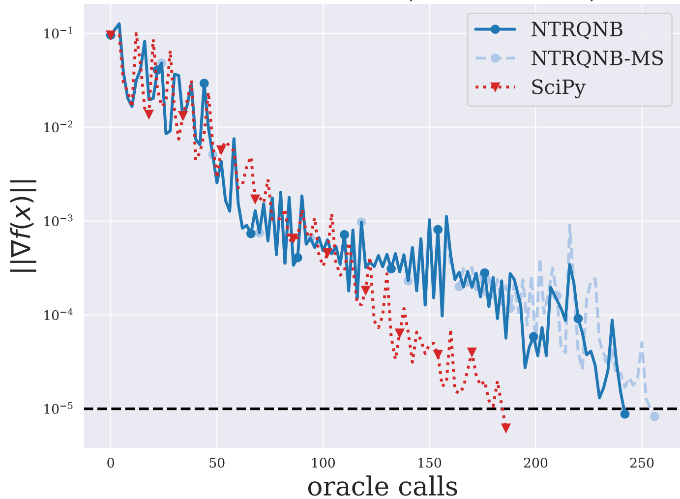
OBSTCLAL ( n = 9604 )
