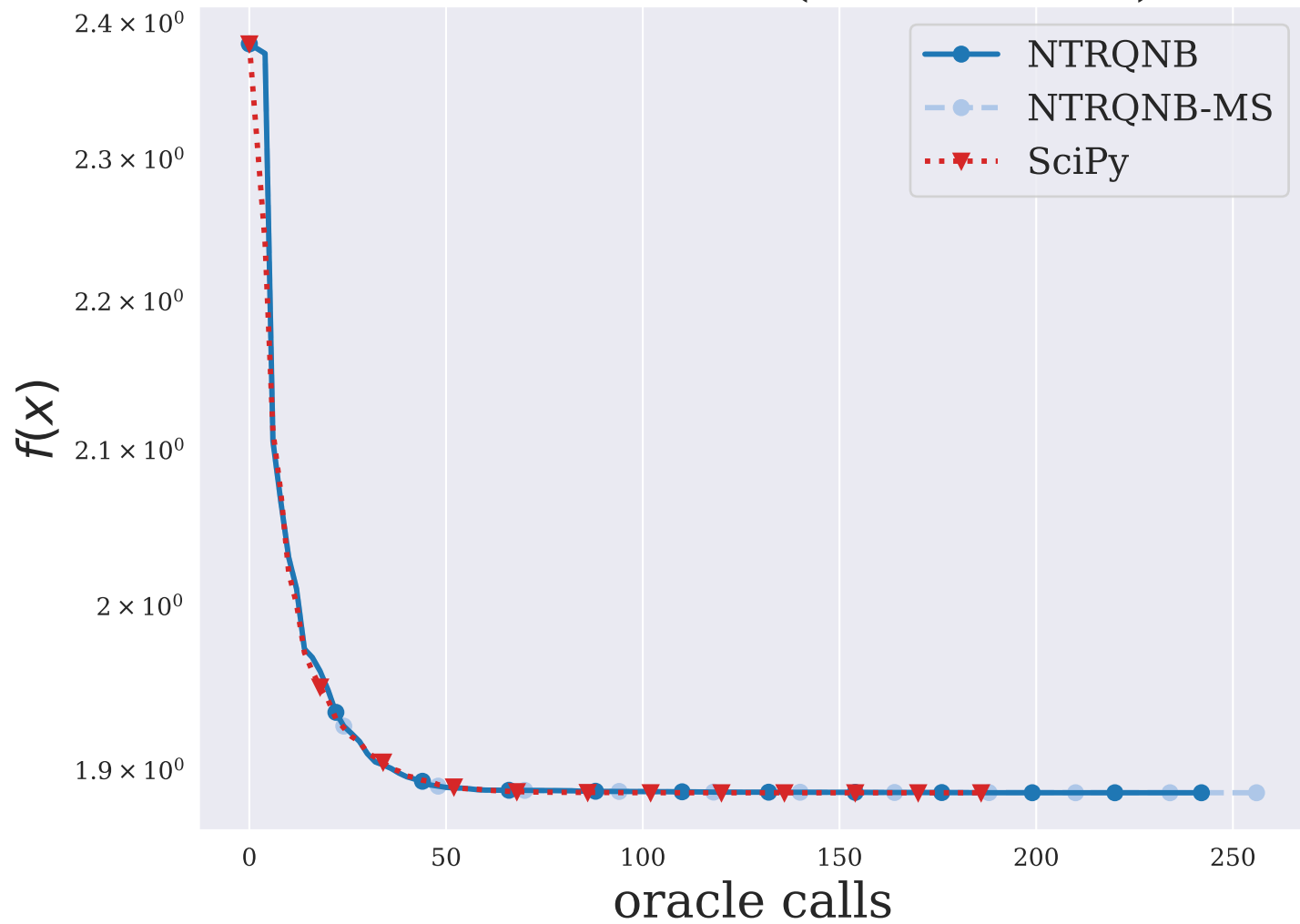
OBSTCLAL ( n = 9604 )
