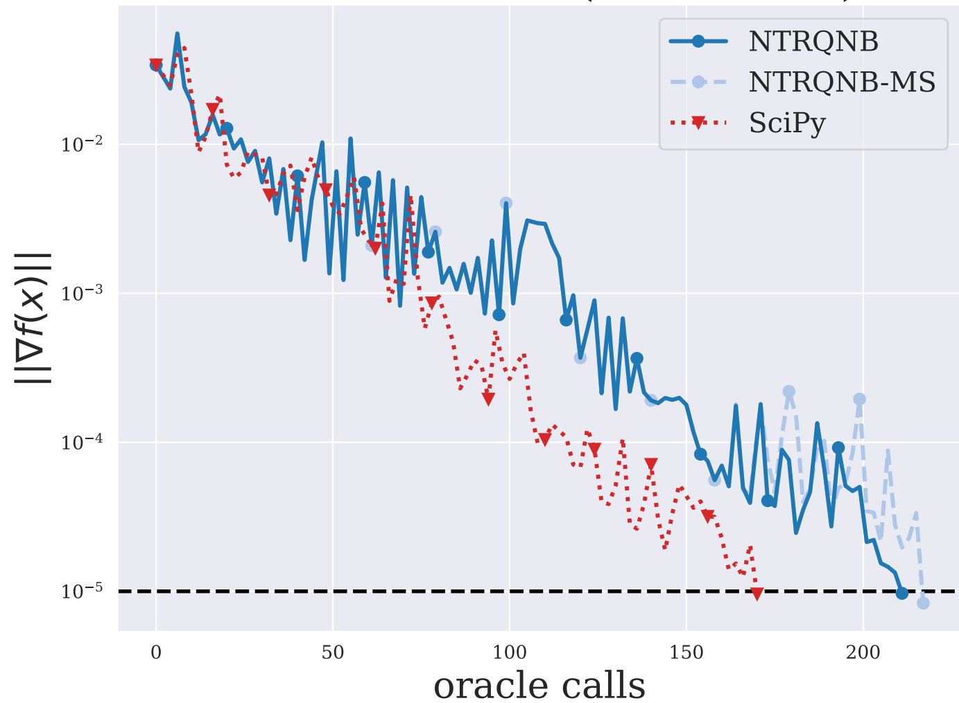
OBSTCLBM ( n = 9604 )
