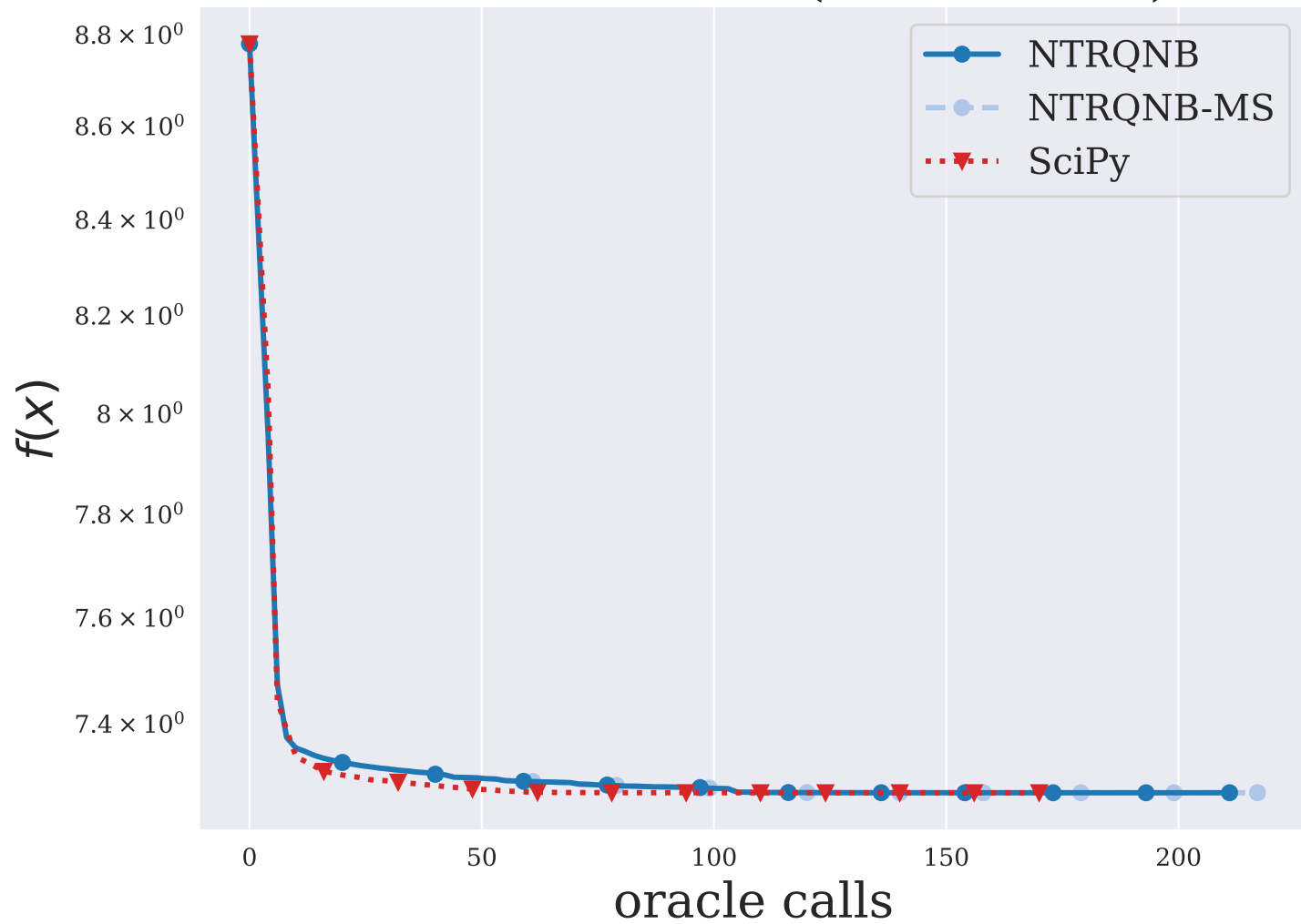
OBSTCLBM ( n = 9604 )
