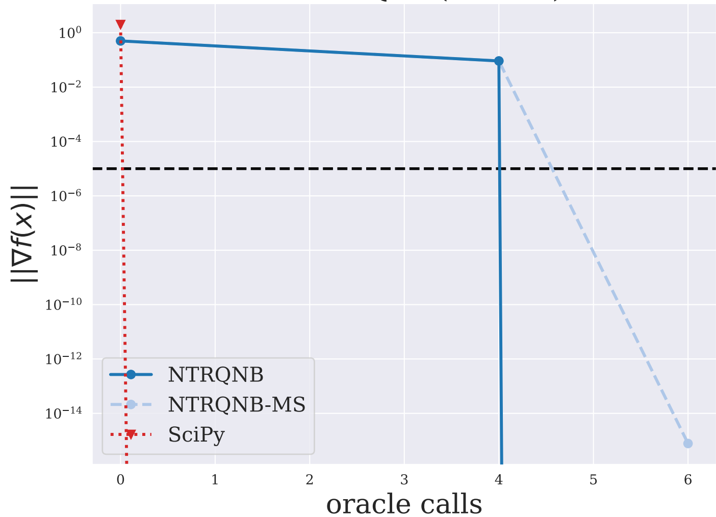
OSLBQP ( n = 8 )
