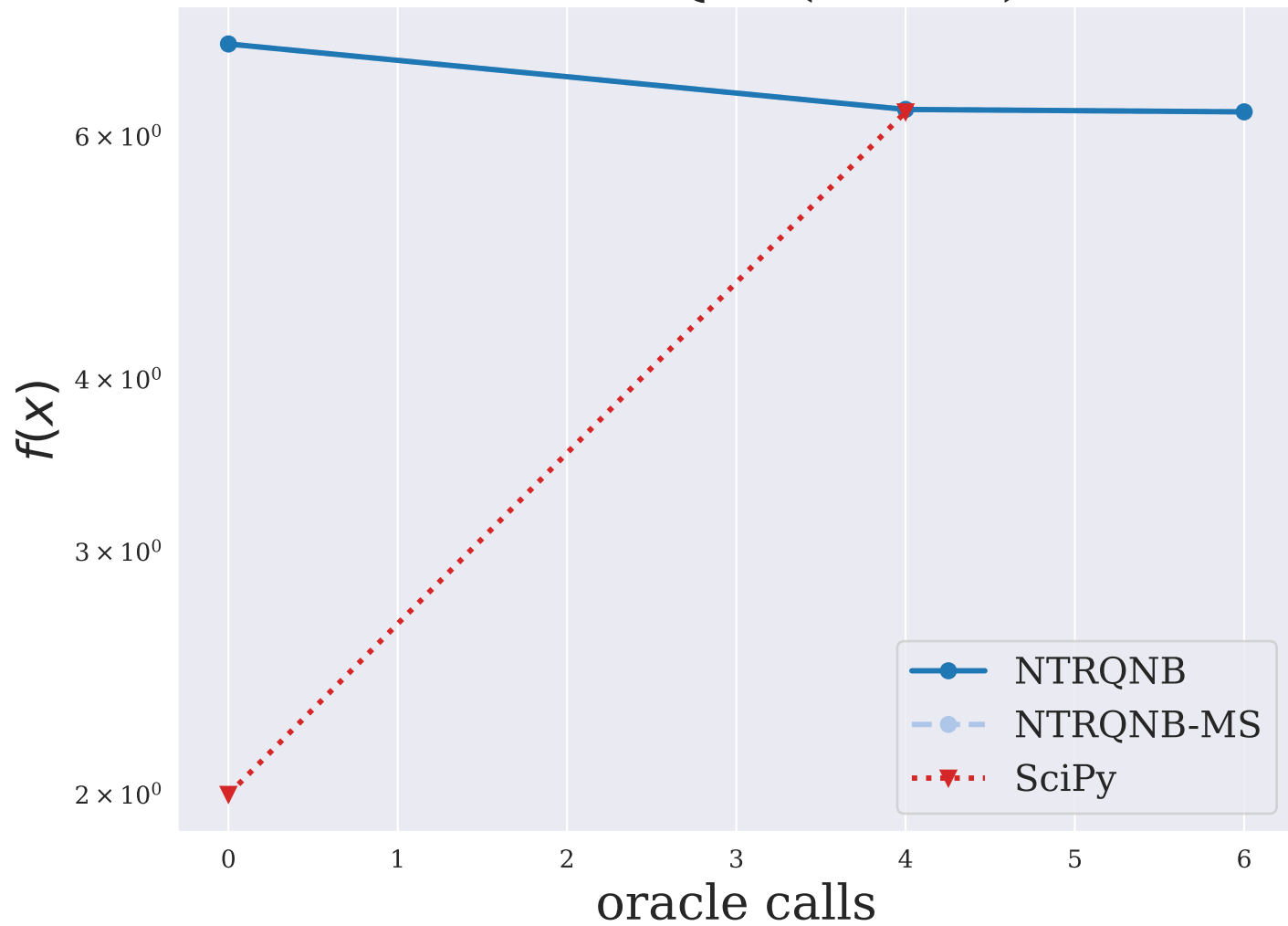
OSLBQP ( n = 8 )
