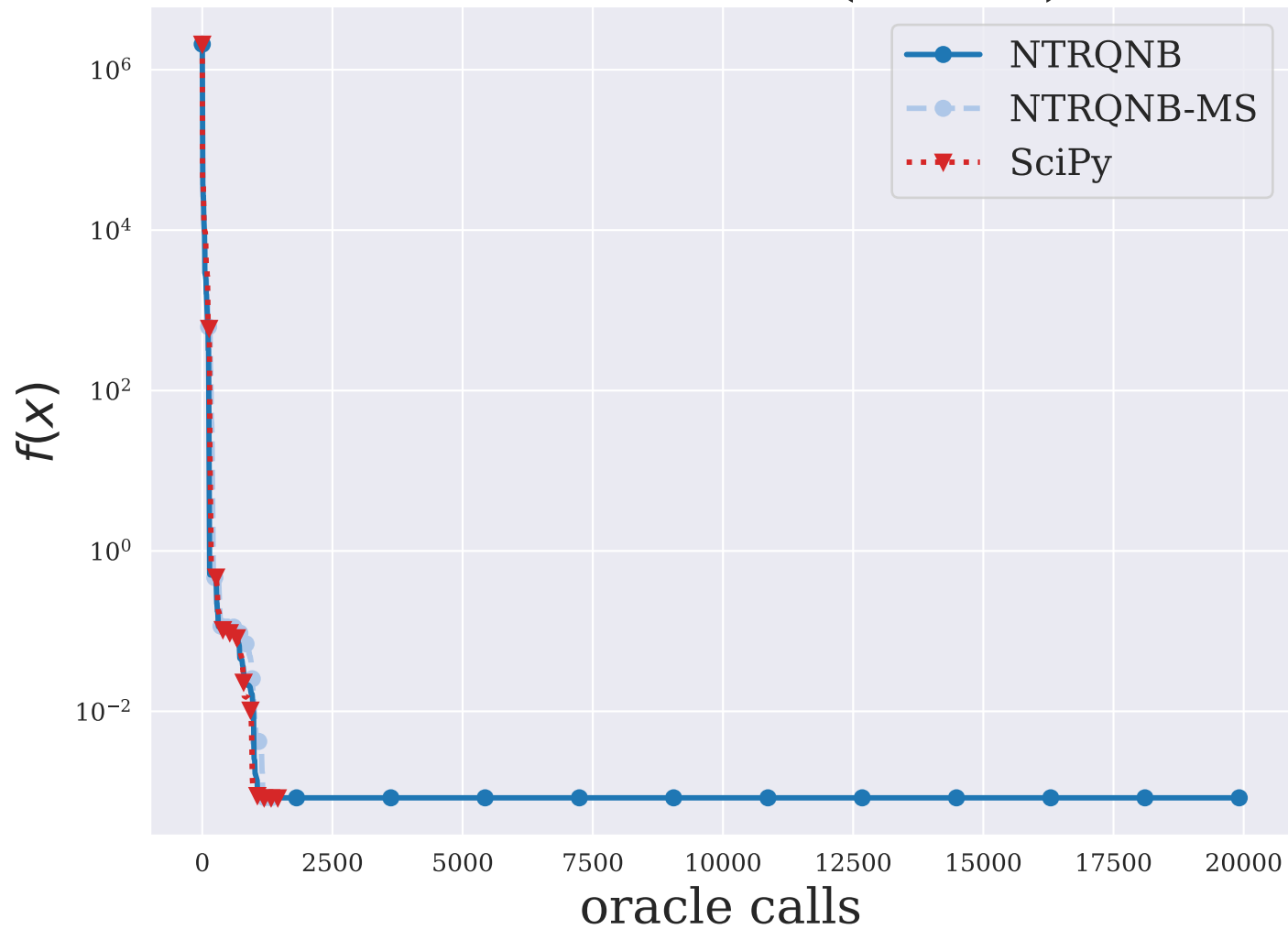
PALMER1E ( n = 8 )
