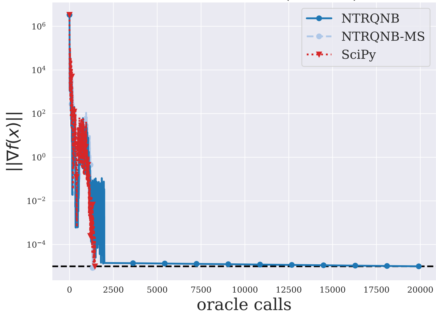
PALMER1E ( n = 8 )
