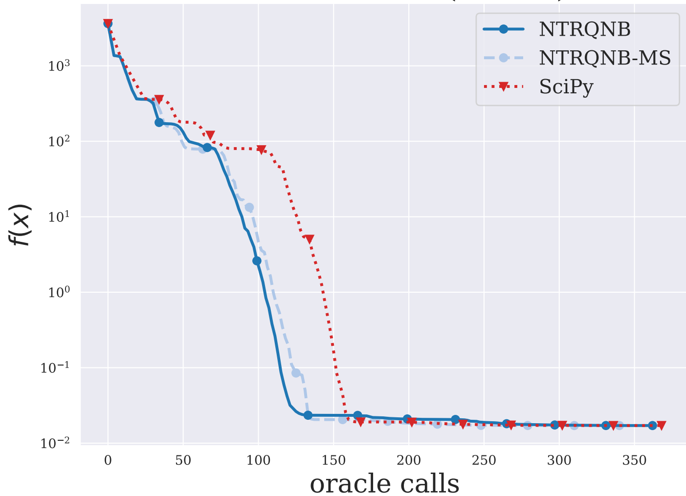
PALMER2A ( n = 6 )
