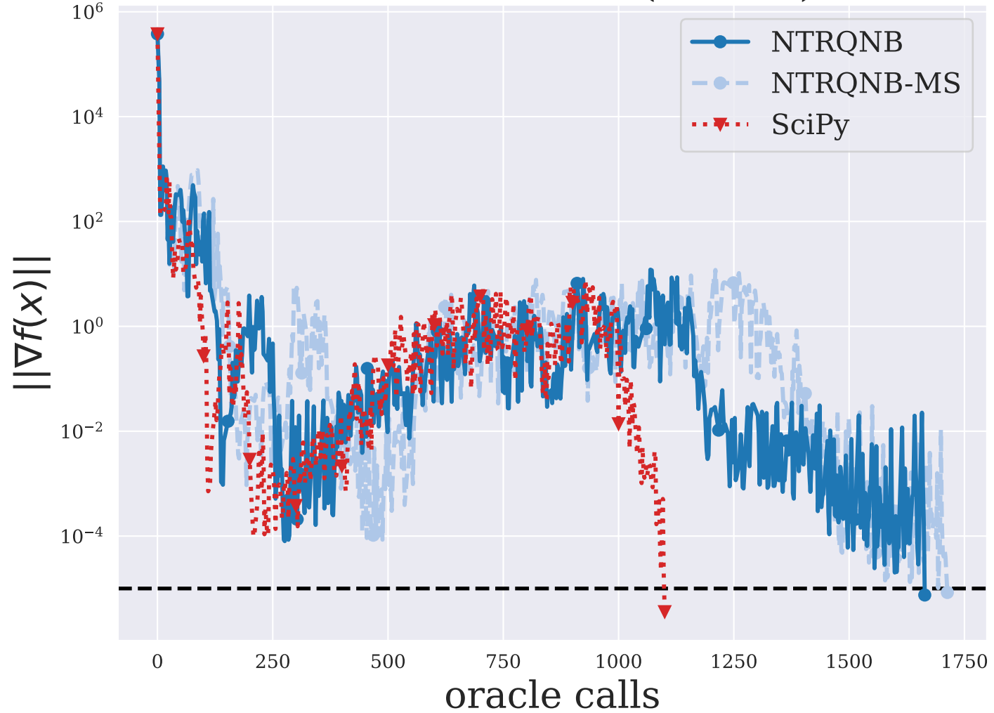
PALMER2E ( n = 8 )
