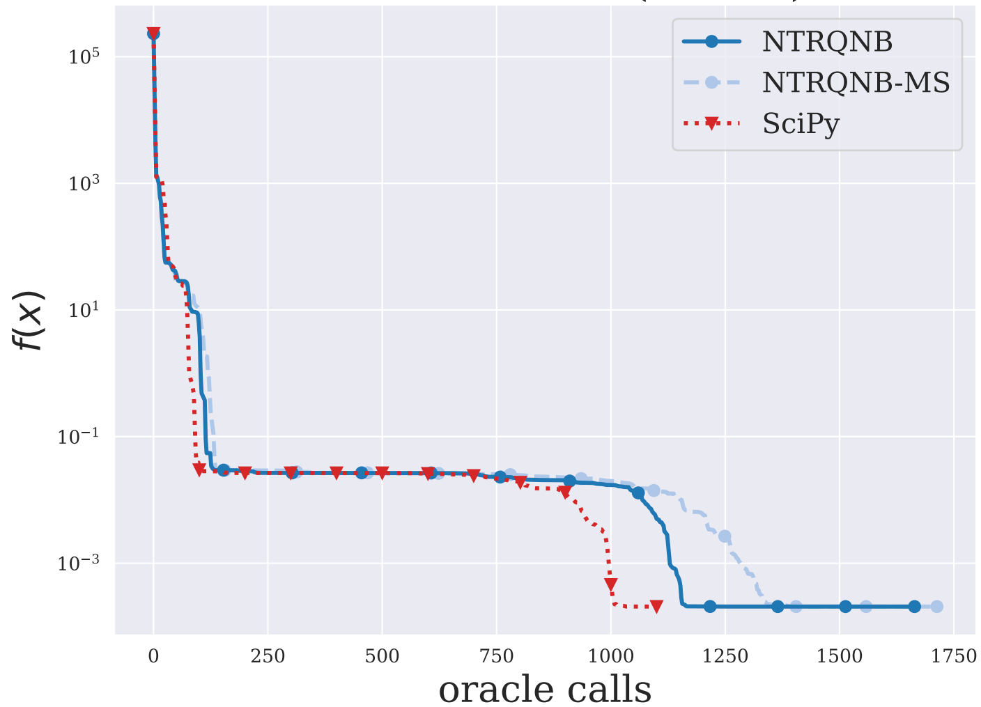
PALMER2E ( n = 8 )
