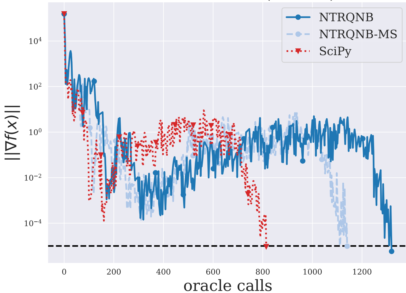
PALMER3E ( n = 8 )
