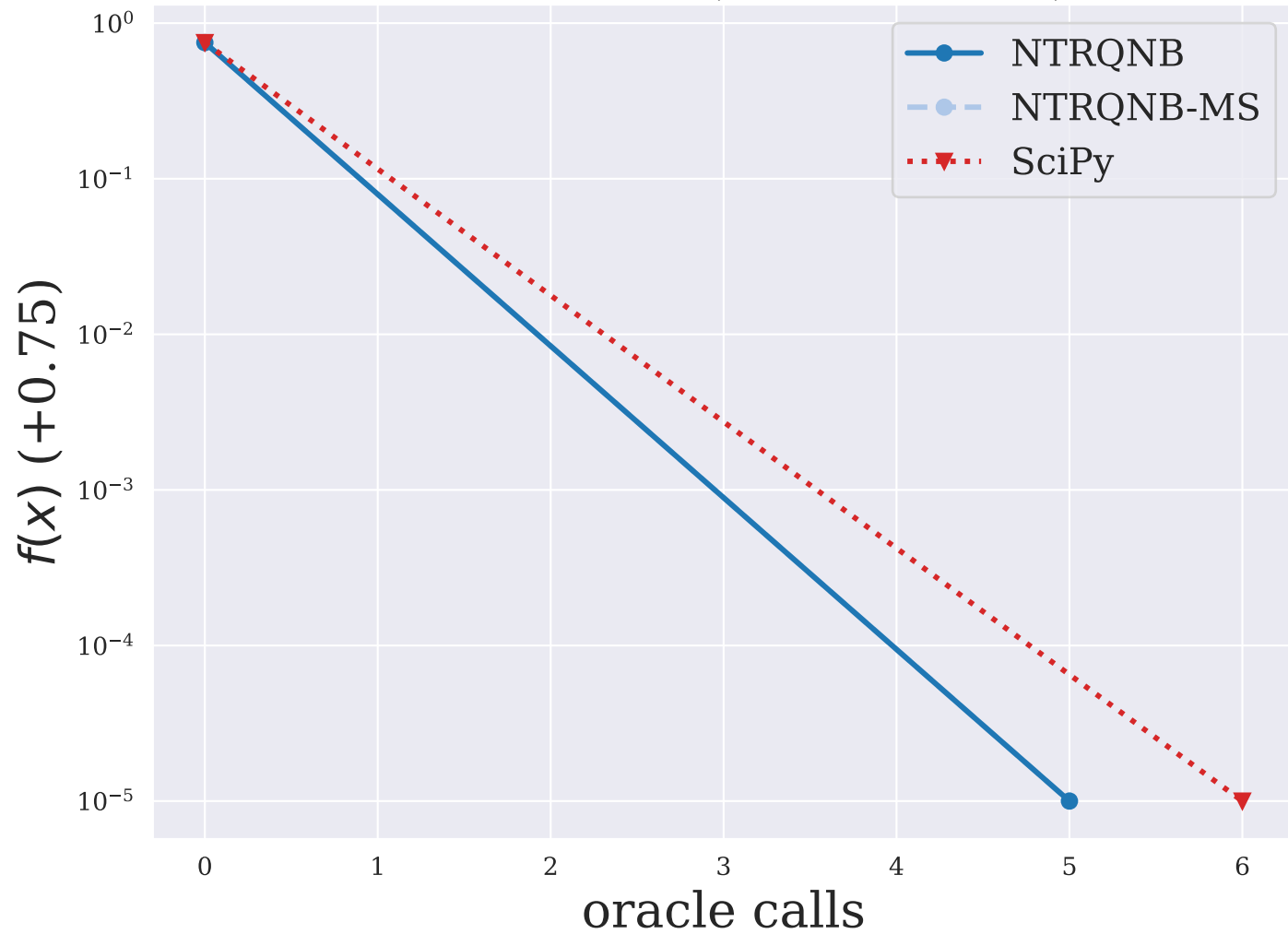
PENTDI ( n = 5000 )
