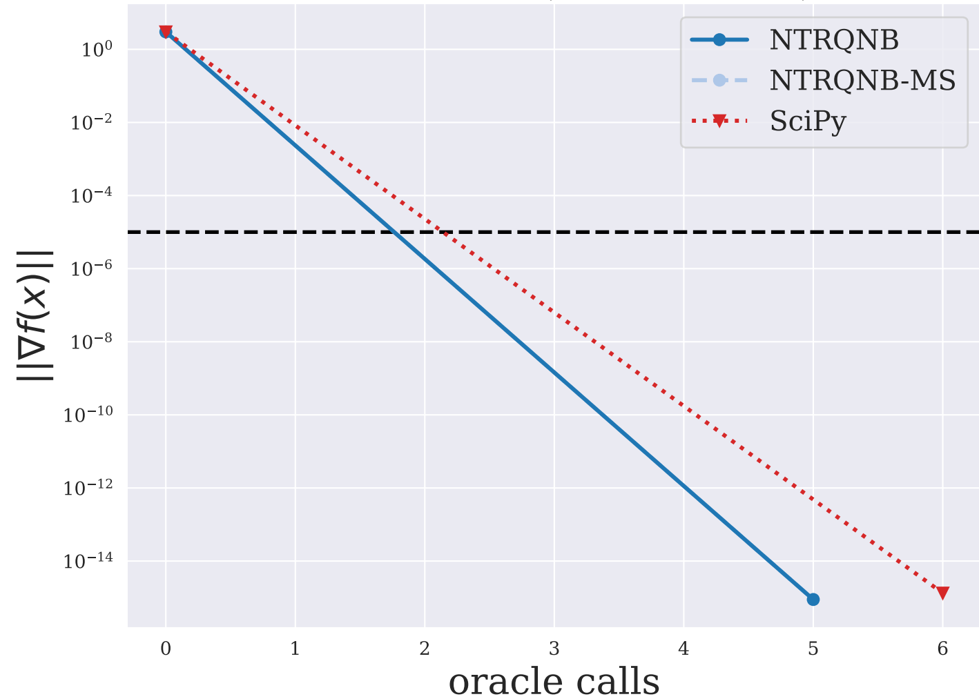
PENTDI ( n = 5000 )
