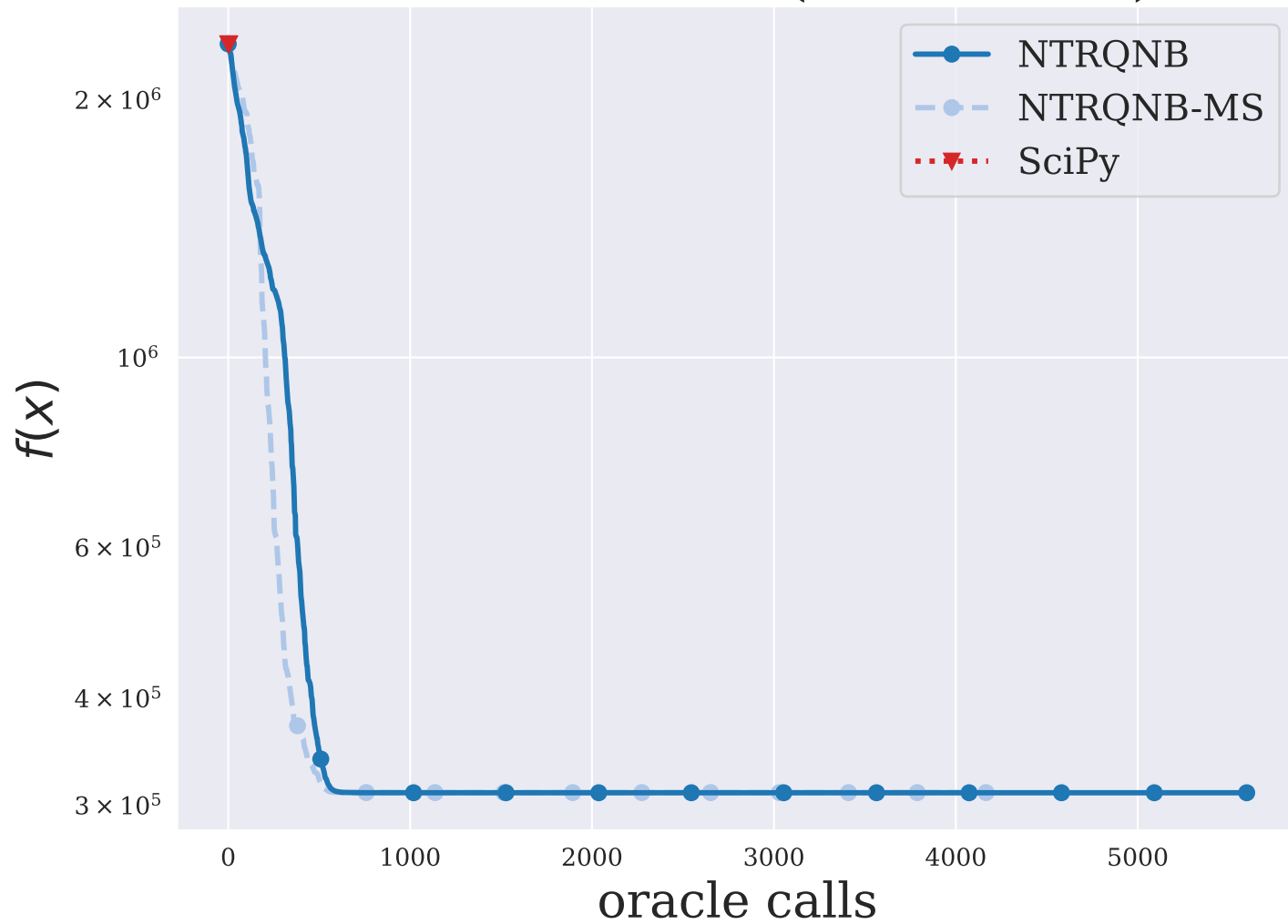
POWELLBC ( n = 1000 )
