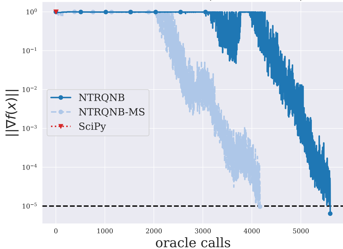
POWELLBC ( n = 1000 )
